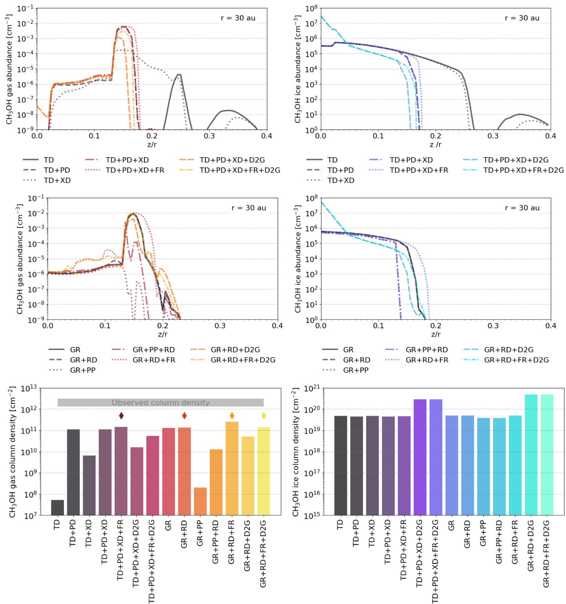
Figure 6. from John D. Ilee et al 2026 Astron. J. 171 doi:10.3847/1538-3881/ae100e https://dx.doi.org/10.3847/1538-3881/ae100e © 2025. The Author(s). Published by the American Astronomical Society.
