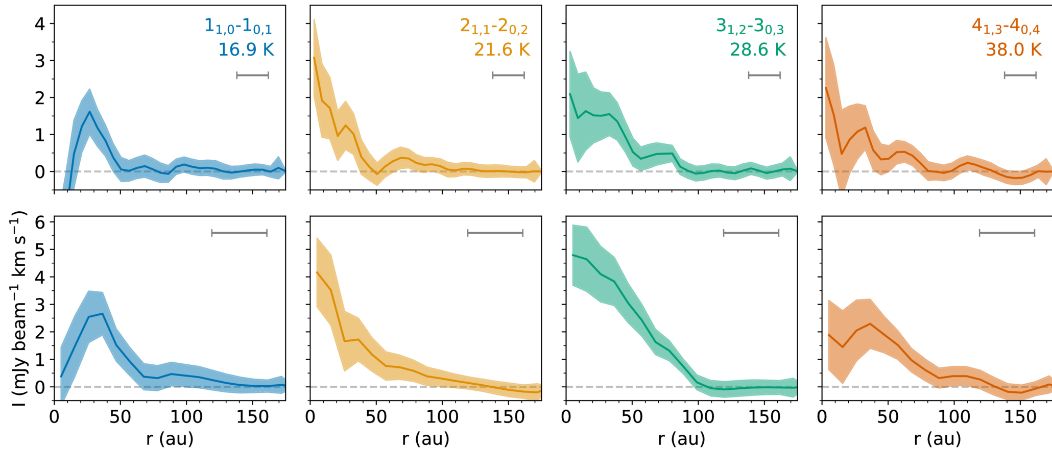
Figure 2. from John D. Ilee et al 2026 Astron. J. 171 doi:10.3847/1538-3881/ae100e https://dx.doi.org/10.3847/1538-3881/ae100e © 2025. The Author(s). Published by the American Astronomical Society.
