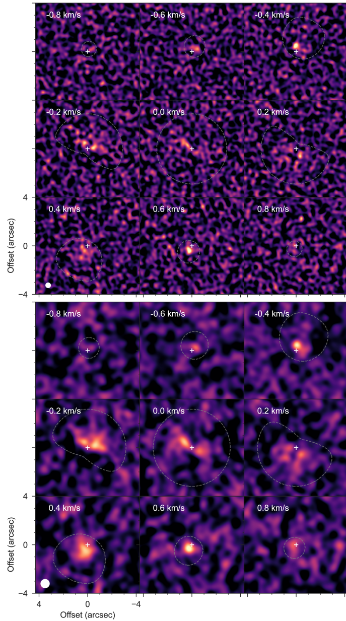
Figure 13. from John D. Ilee et al 2026 Astron. J. 171 doi:10.3847/1538-3881/ae100e https://dx.doi.org/10.3847/1538-3881/ae100e © 2025. The Author(s). Published by the American Astronomical Society.
