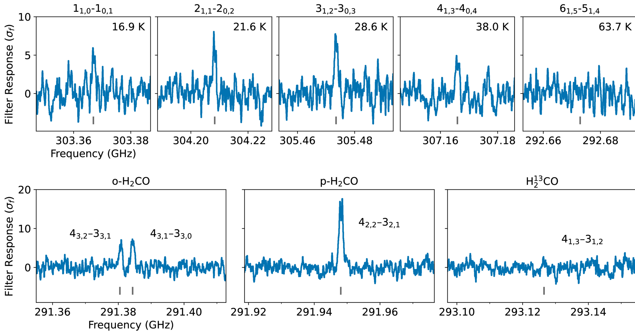
Figure 12. from John D. Ilee et al 2026 Astron. J. 171 doi:10.3847/1538-3881/ae100e https://dx.doi.org/10.3847/1538-3881/ae100e © 2025. The Author(s). Published by the American Astronomical Society.
