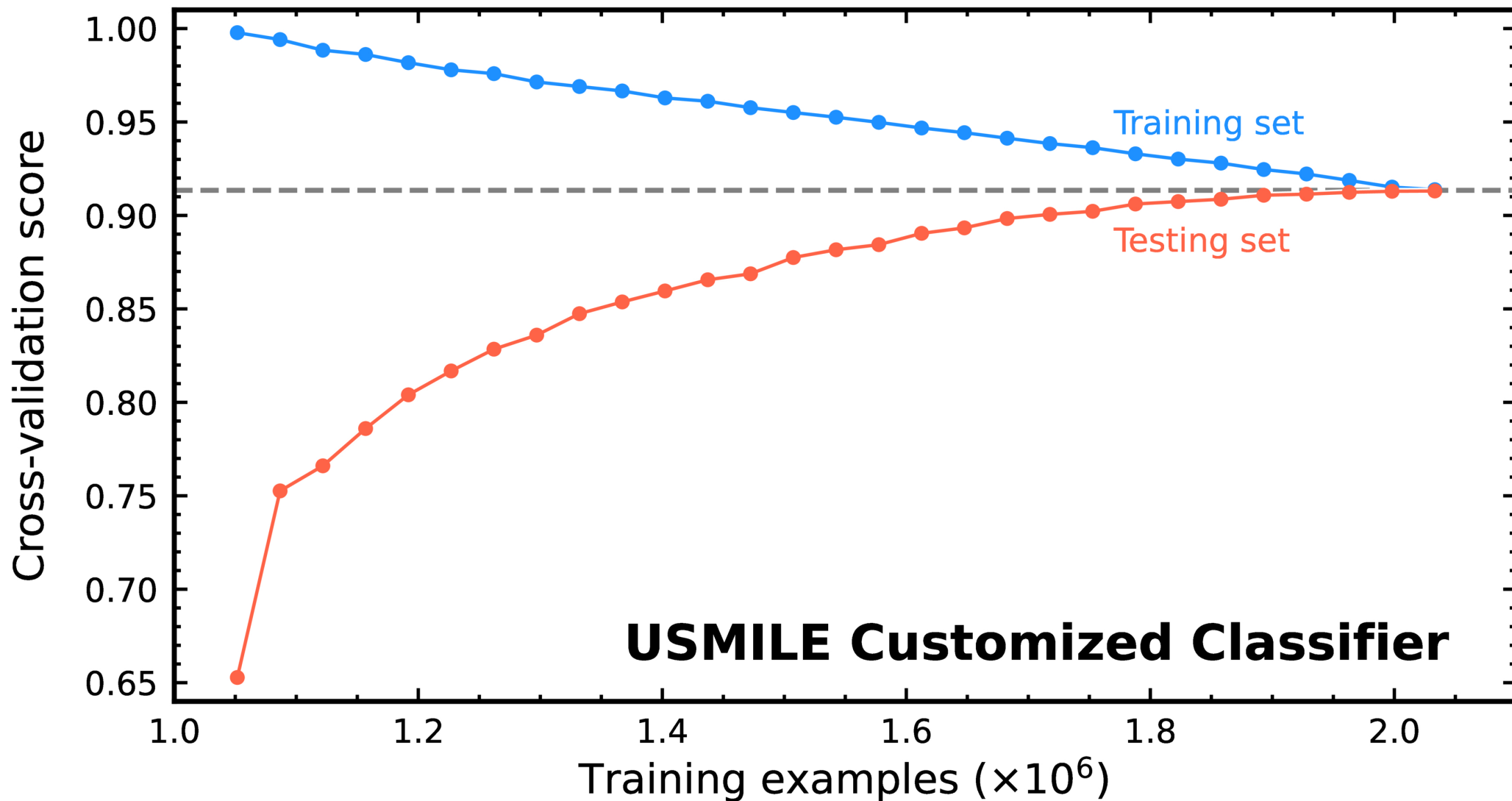
Figure 5. from Zhoujian Zhang et al 2025 Astron. J. 170 doi:10.3847/1538-3881/ae100b https://dx.doi.org/10.3847/1538-3881/ae100b © 2025. The Author(s). Published by the American Astronomical Society.
