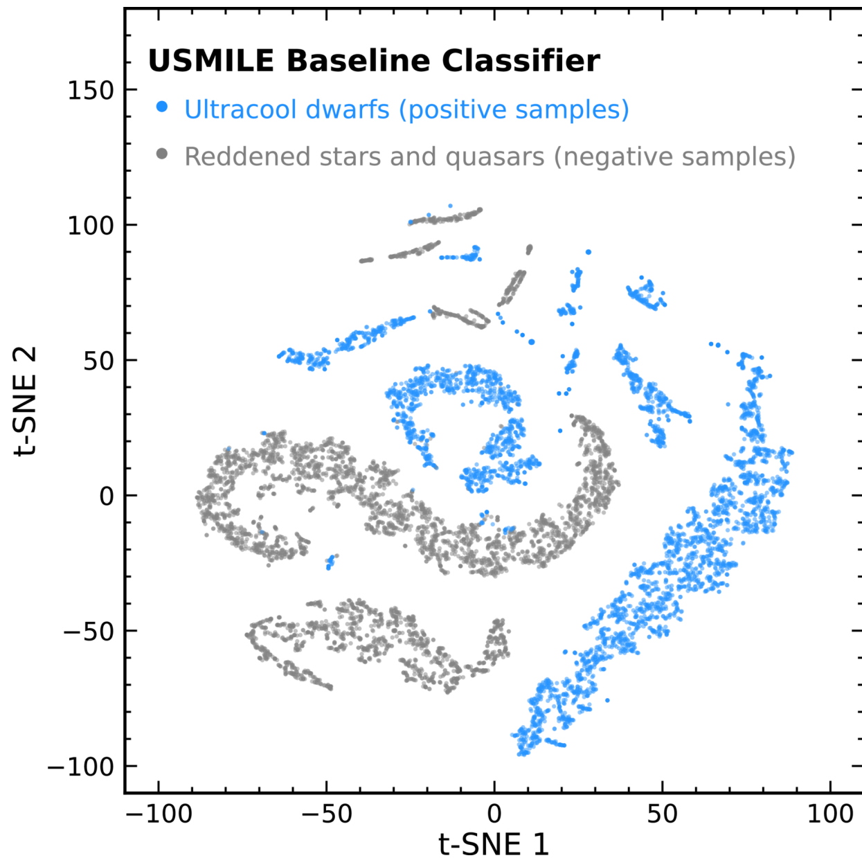
Figure 2. from Zhoujian Zhang et al 2025 Astron. J. 170 doi:10.3847/1538-3881/ae100b https://dx.doi.org/10.3847/1538-3881/ae100b © 2025. The Author(s). Published by the American Astronomical Society.
