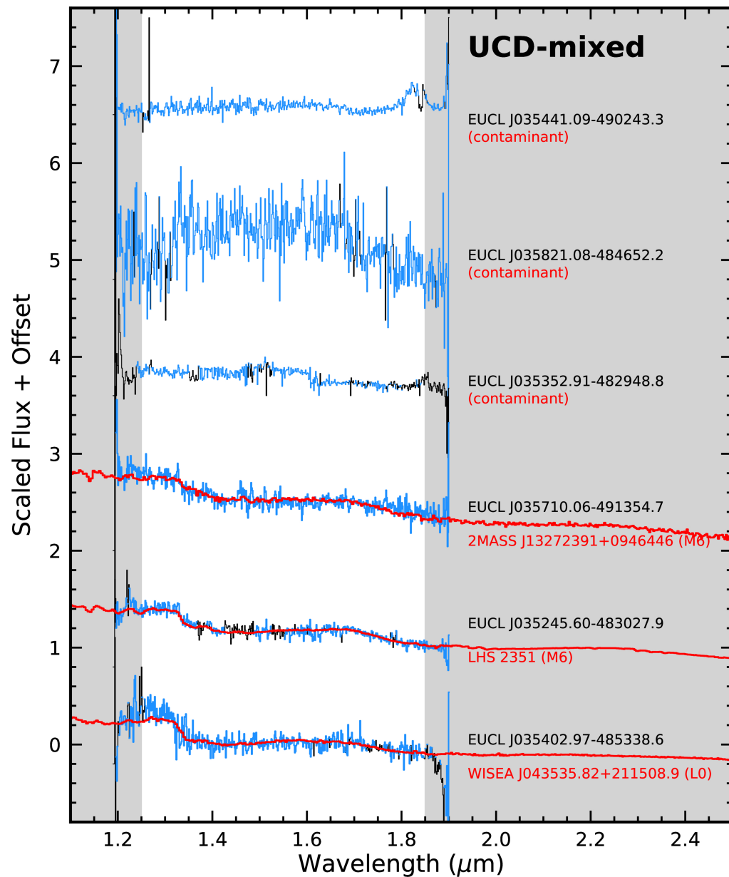
Figure 14. from Zhoujian Zhang et al 2025 Astron. J. 170 doi:10.3847/1538-3881/ae100b https://dx.doi.org/10.3847/1538-3881/ae100b © 2025. The Author(s). Published by the American Astronomical Society.
