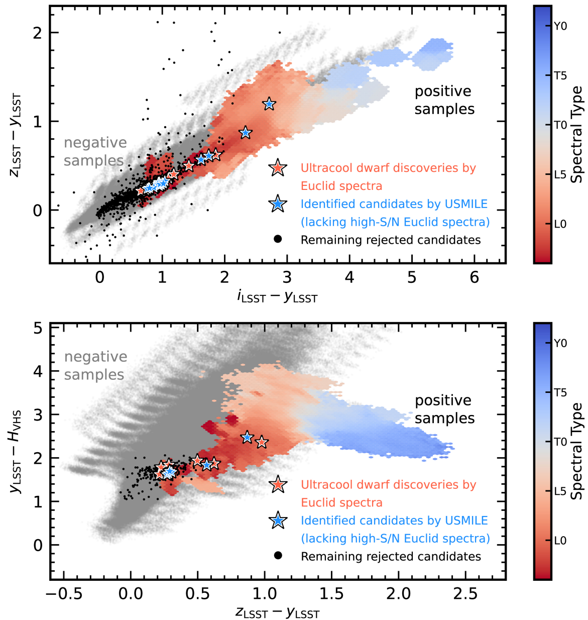
Figure 11. from Zhoujian Zhang et al 2025 Astron. J. 170 doi:10.3847/1538-3881/ae100b https://dx.doi.org/10.3847/1538-3881/ae100b © 2025. The Author(s). Published by the American Astronomical Society.
