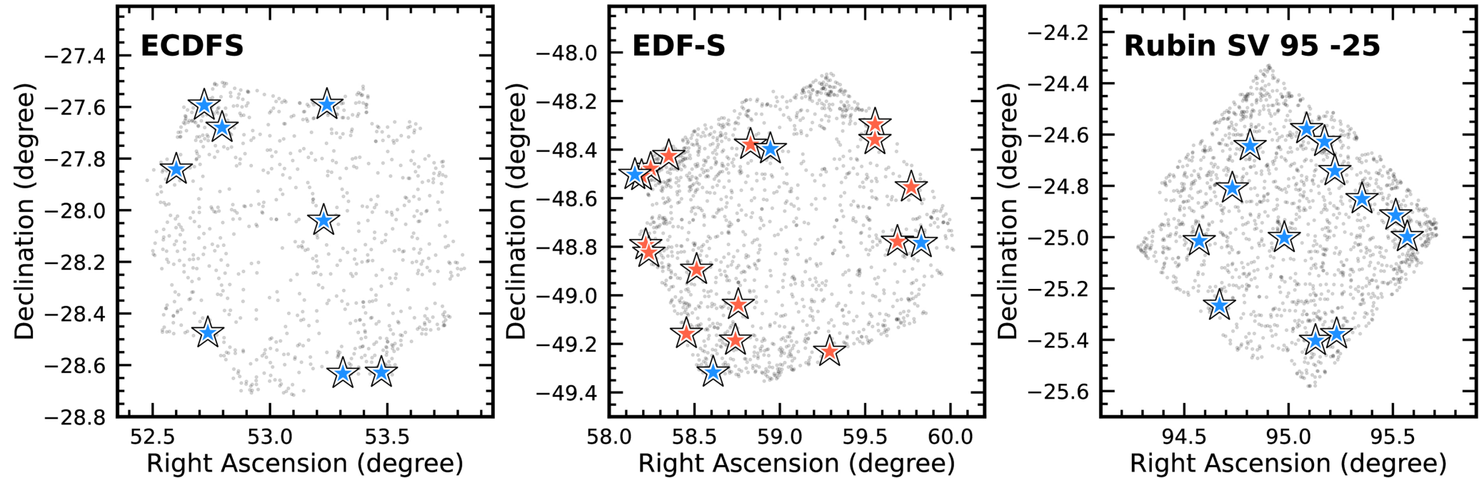
Figure 10. from Zhoujian Zhang et al 2025 Astron. J. 170 doi:10.3847/1538-3881/ae100b https://dx.doi.org/10.3847/1538-3881/ae100b © 2025. The Author(s). Published by the American Astronomical Society.
