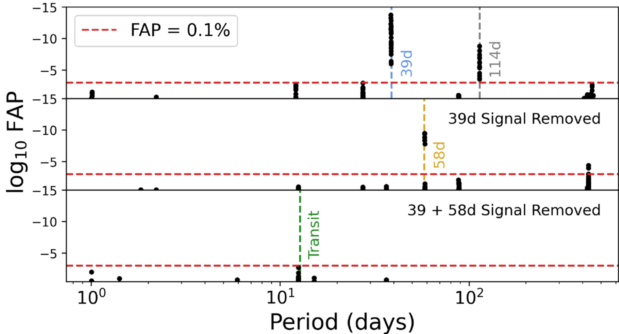
Figure 7. from Madison Brady et al 2025 Astron. J. 170 doi:10.3847/1538-3881/ae0f98 https://dx.doi.org/10.3847/1538-3881/ae0f98 © 2025. The Author(s). Published by the American Astronomical Society.
