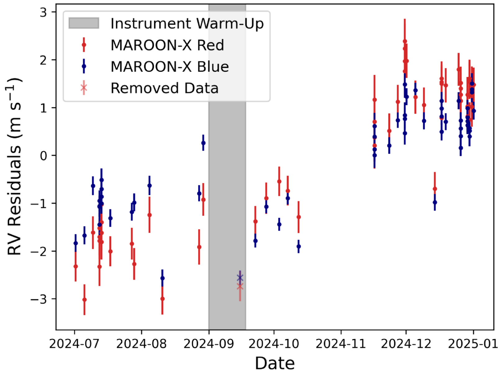
Figure 3. from Madison Brady et al 2025 Astron. J. 170 doi:10.3847/1538-3881/ae0f98 https://dx.doi.org/10.3847/1538-3881/ae0f98 © 2025. The Author(s). Published by the American Astronomical Society.
