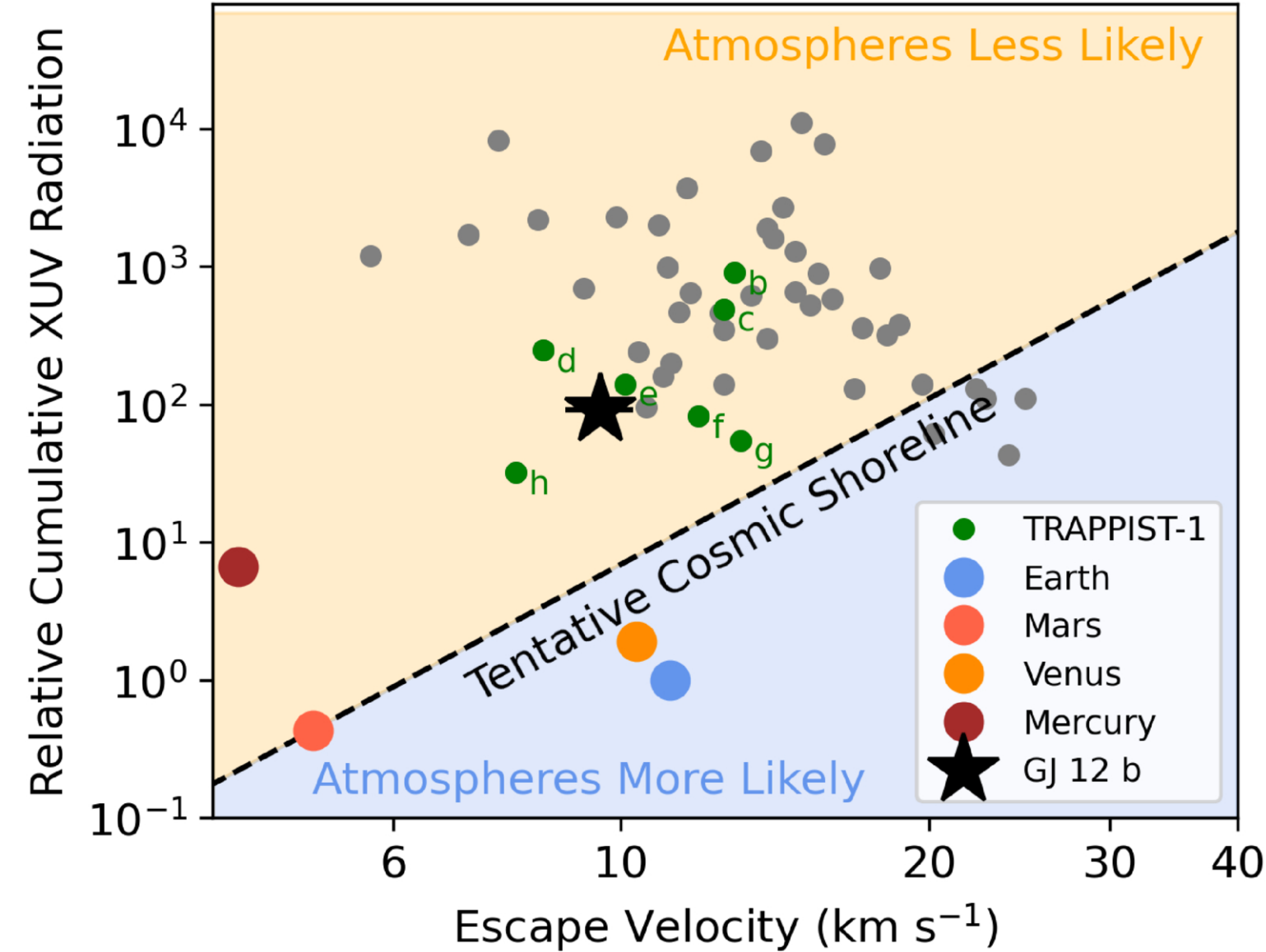
Figure 11. from Madison Brady et al 2025 Astron. J. 170 doi:10.3847/1538-3881/ae0f98 https://dx.doi.org/10.3847/1538-3881/ae0f98 © 2025. The Author(s). Published by the American Astronomical Society.
