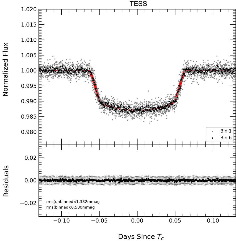
Figure 6. from E. Sonbas et al 2025 Astron. J. 170 doi:10.3847/1538-3881/ae0f19 https://dx.doi.org/10.3847/1538-3881/ae0f19 © 2025. The Author(s). Published by the American Astronomical Society.
