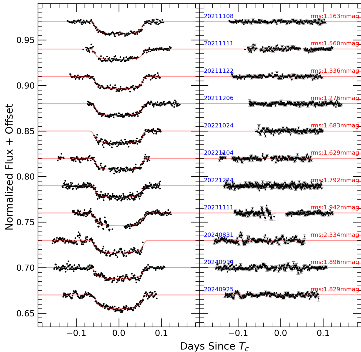
Figure 2. from E. Sonbas et al 2025 Astron. J. 170 doi:10.3847/1538-3881/ae0f19 https://dx.doi.org/10.3847/1538-3881/ae0f19 © 2025. The Author(s). Published by the American Astronomical Society.
