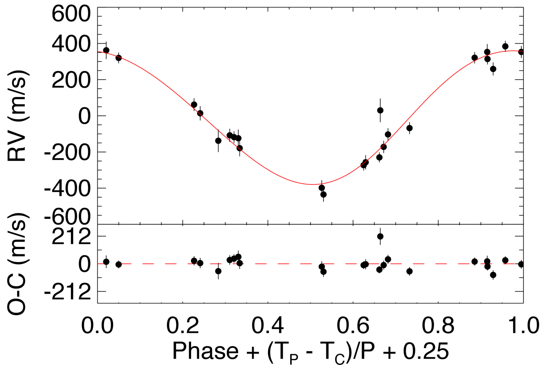
Figure 11. from E. Sonbas et al 2025 Astron. J. 170 doi:10.3847/1538-3881/ae0f19 https://dx.doi.org/10.3847/1538-3881/ae0f19 © 2025. The Author(s). Published by the American Astronomical Society.
