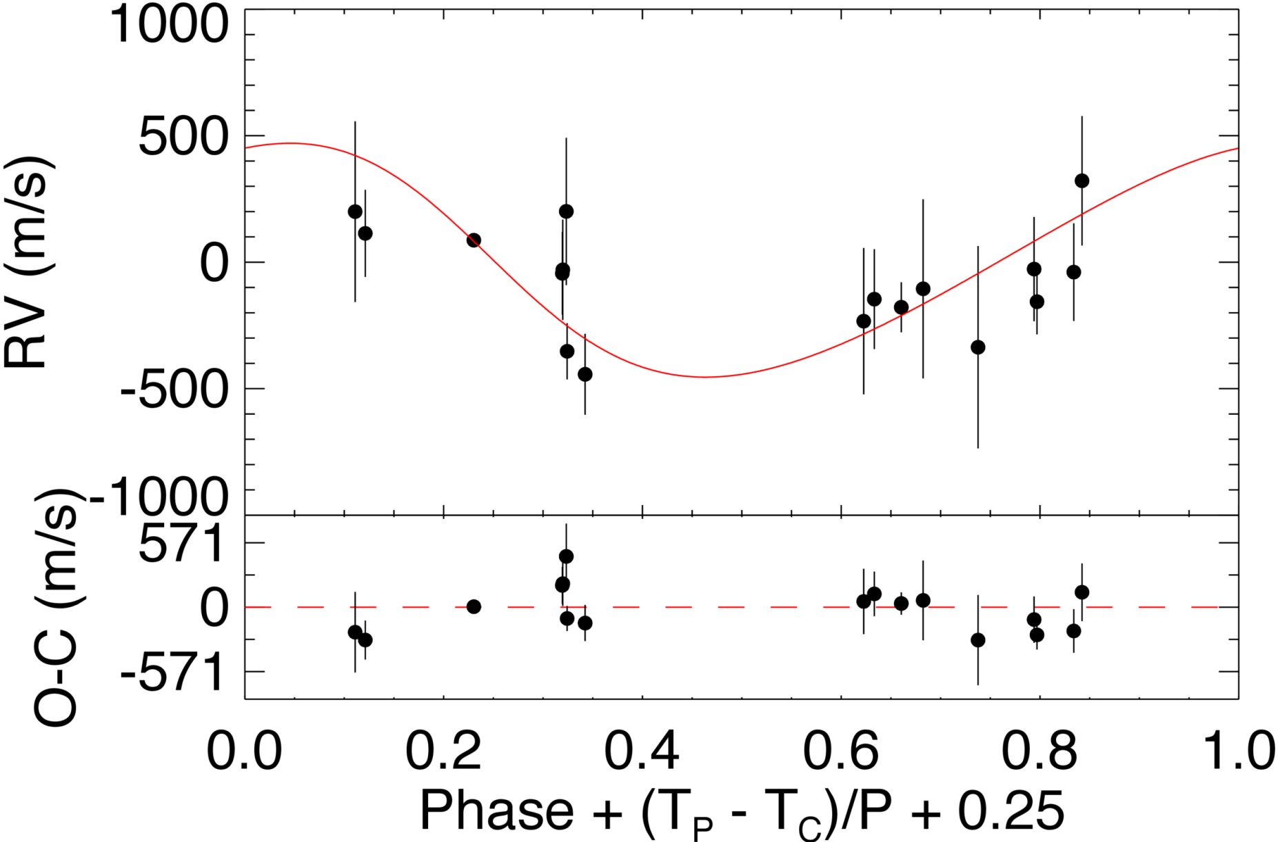
Figure 10. from E. Sonbas et al 2025 Astron. J. 170 doi:10.3847/1538-3881/ae0f19 https://dx.doi.org/10.3847/1538-3881/ae0f19 © 2025. The Author(s). Published by the American Astronomical Society.
