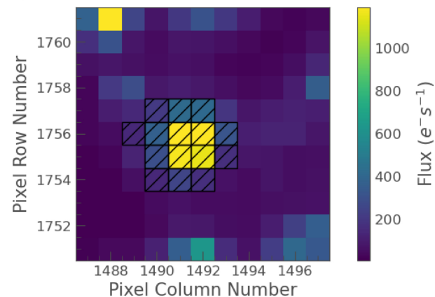
(a) TOI-1516 in sector 58.
