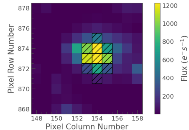
(c) HAT-P-16 in sector 17.
