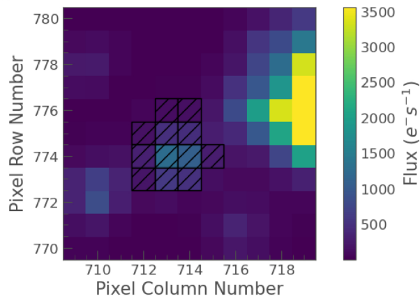
(b) TOI-2046 in sector 58.
