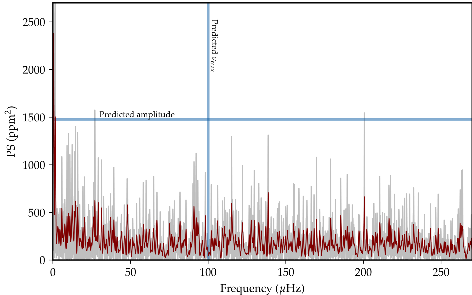
Figure 5. from Daniel Hey et al 2025 Astron. J. 170 doi:10.3847/1538-3881/ae0e25 https://dx.doi.org/10.3847/1538-3881/ae0e25 © 2025. The Author(s). Published by the American Astronomical Society.
