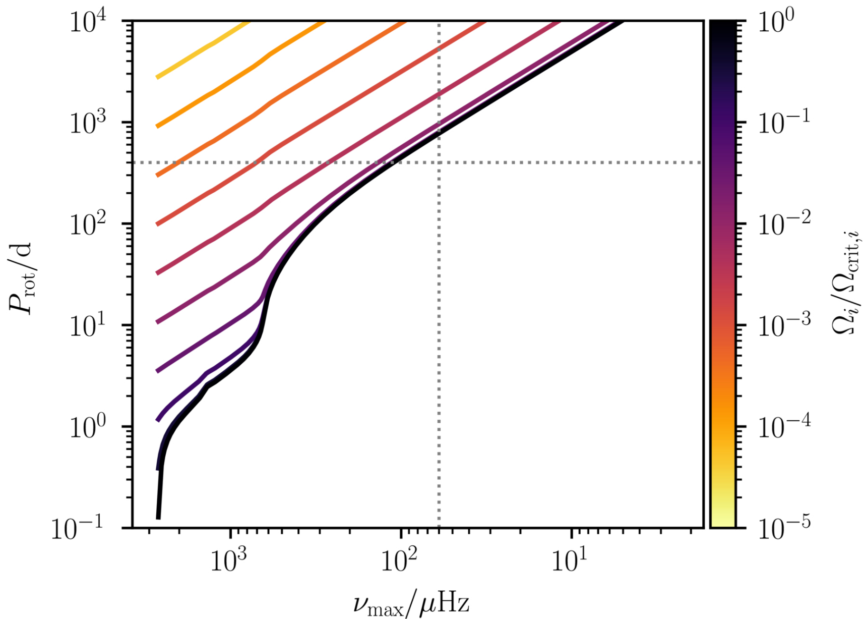
Figure 4. from Daniel Hey et al 2025 Astron. J. 170 doi:10.3847/1538-3881/ae0e25 https://dx.doi.org/10.3847/1538-3881/ae0e25 © 2025. The Author(s). Published by the American Astronomical Society.
