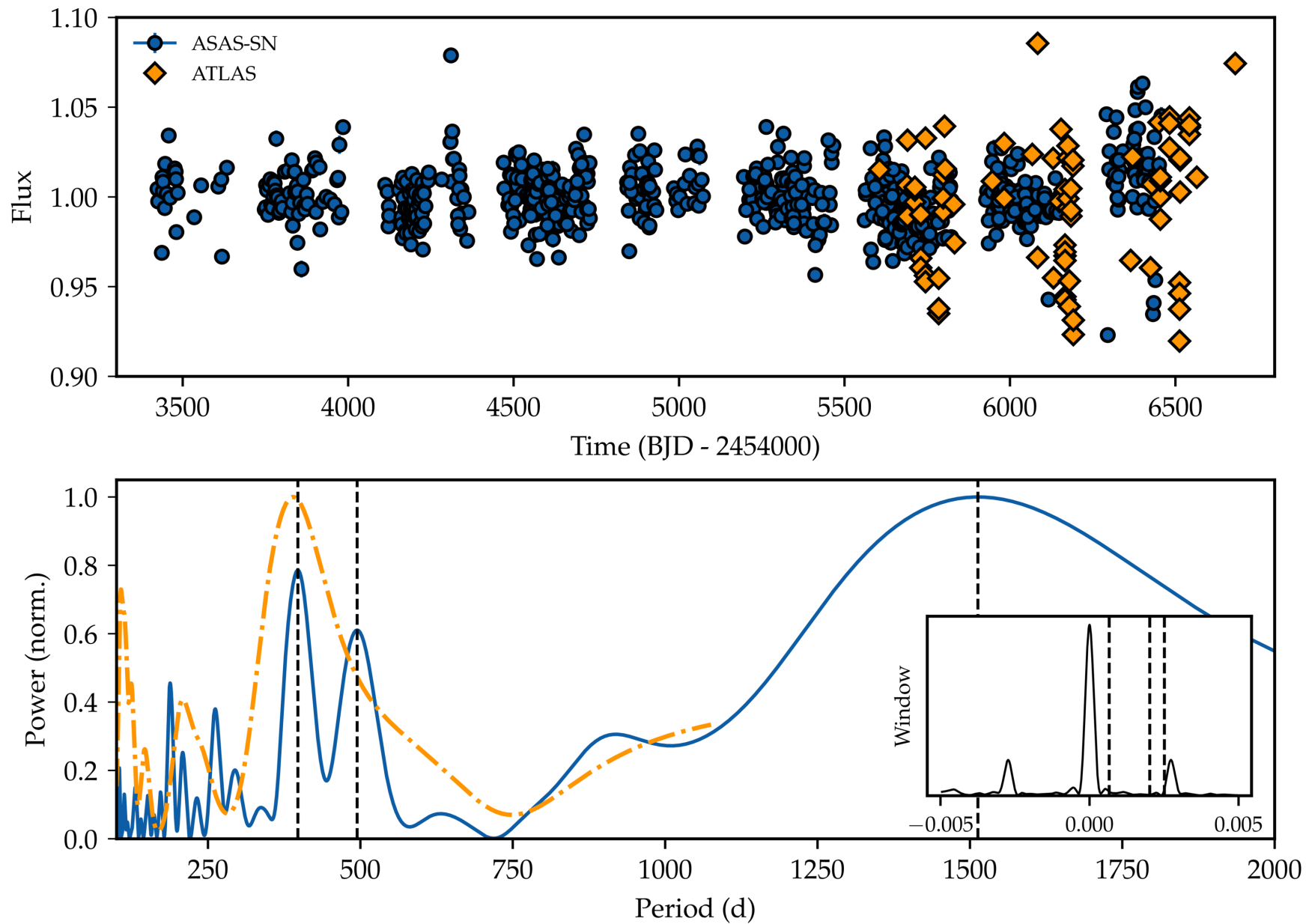
Figure 3. from Daniel Hey et al 2025 Astron. J. 170 doi:10.3847/1538-3881/ae0e25 https://dx.doi.org/10.3847/1538-3881/ae0e25 © 2025. The Author(s). Published by the American Astronomical Society.
