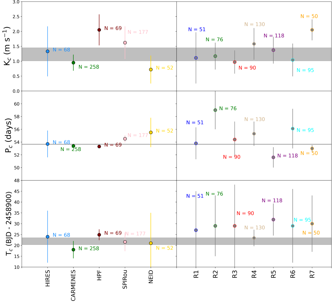
Figure 9. from Corey Beard et al 2025 Astron. J. 170 doi:10.3847/1538-3881/ae0e20 https://dx.doi.org/10.3847/1538-3881/ae0e20 © 2025. The Author(s). Published by the American Astronomical Society.
