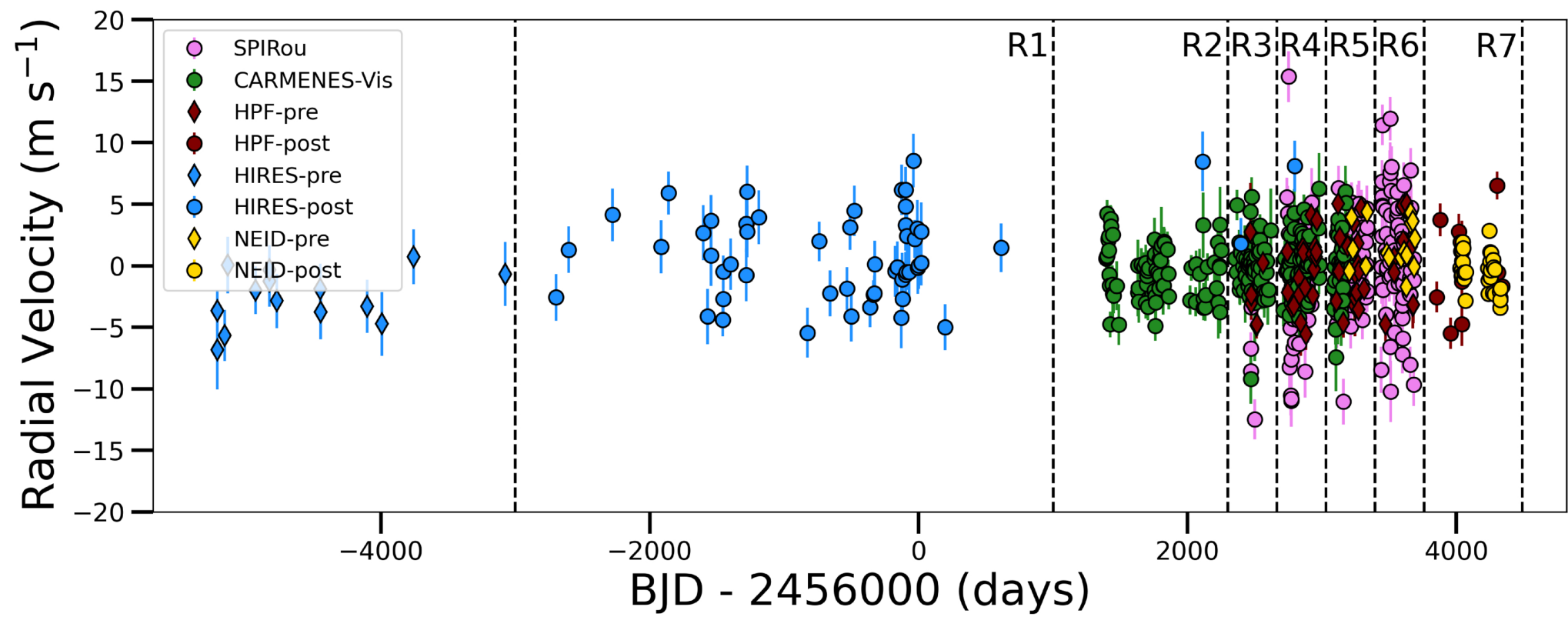
Figure 8. from Corey Beard et al 2025 Astron. J. 170 doi:10.3847/1538-3881/ae0e20 https://dx.doi.org/10.3847/1538-3881/ae0e20 © 2025. The Author(s). Published by the American Astronomical Society.
