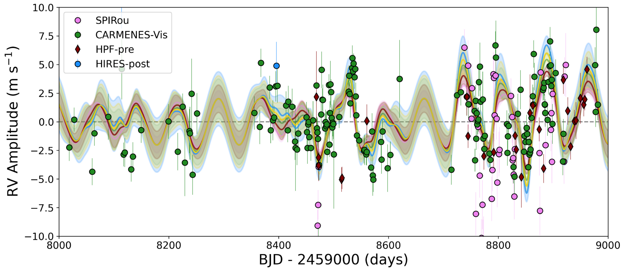
Figure 7. from Corey Beard et al 2025 Astron. J. 170 doi:10.3847/1538-3881/ae0e20 https://dx.doi.org/10.3847/1538-3881/ae0e20 © 2025. The Author(s). Published by the American Astronomical Society.
