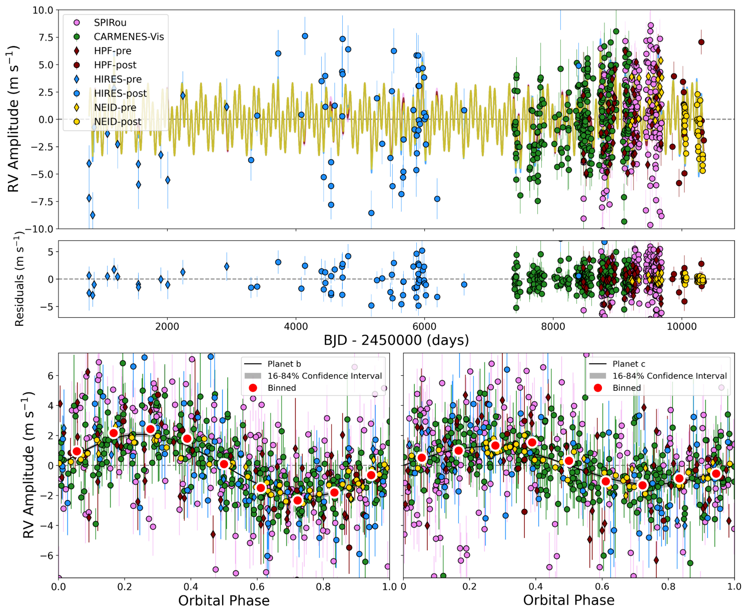
Figure 6. from Corey Beard et al 2025 Astron. J. 170 doi:10.3847/1538-3881/ae0e20 https://dx.doi.org/10.3847/1538-3881/ae0e20 © 2025. The Author(s). Published by the American Astronomical Society.
