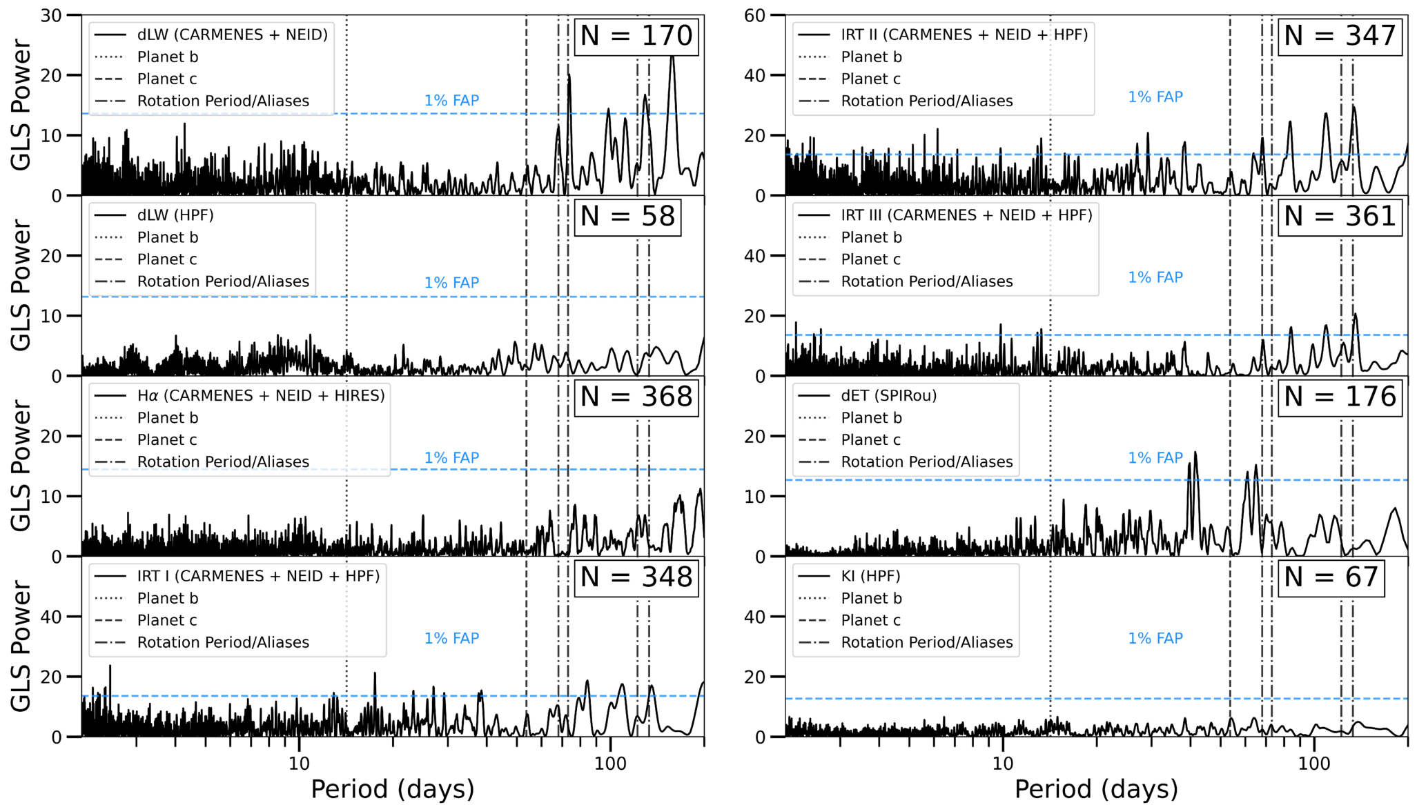
Figure 5. from Corey Beard et al 2025 Astron. J. 170 doi:10.3847/1538-3881/ae0e20 https://dx.doi.org/10.3847/1538-3881/ae0e20 © 2025. The Author(s). Published by the American Astronomical Society.
