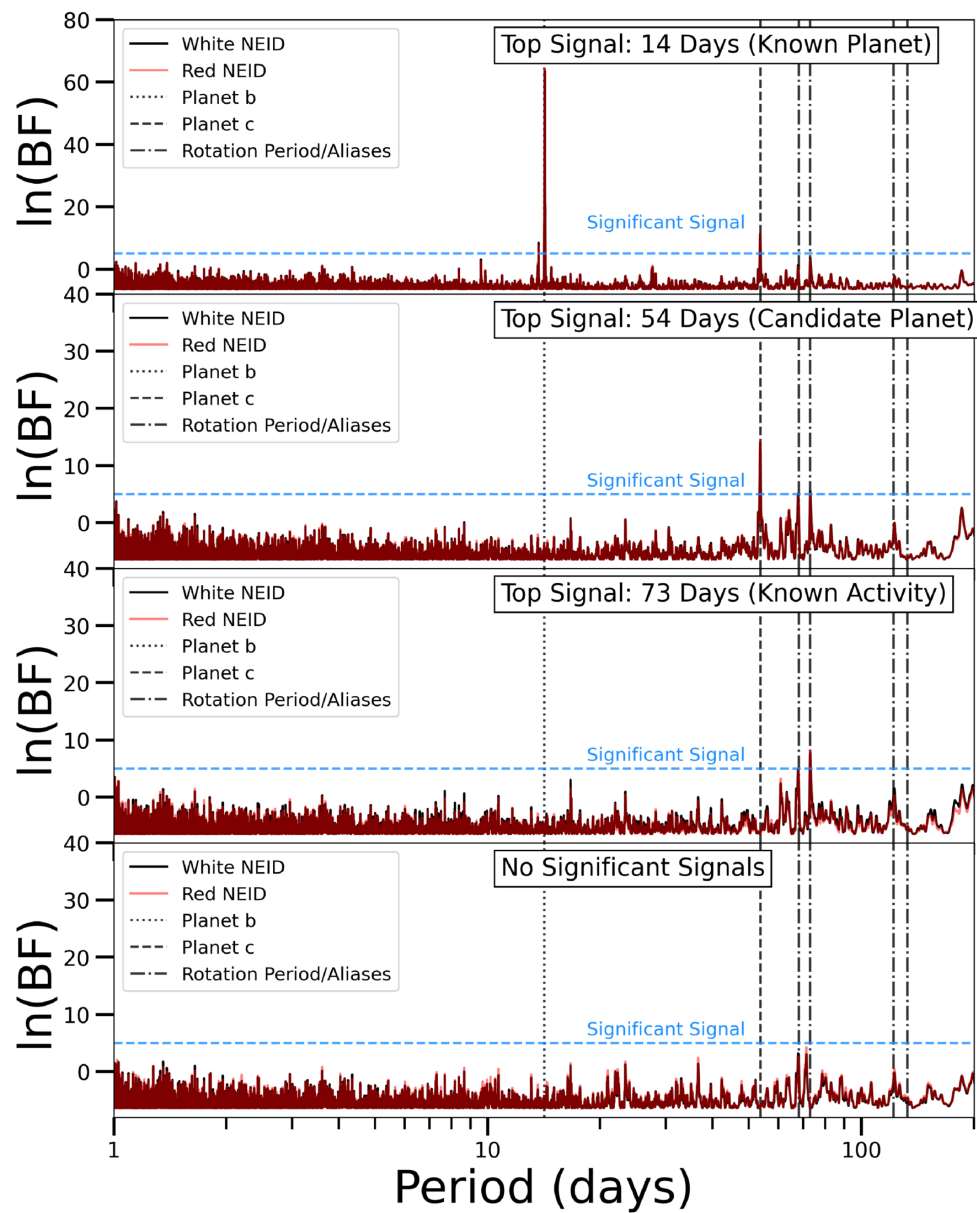
Figure 4. from Corey Beard et al 2025 Astron. J. 170 doi:10.3847/1538-3881/ae0e20 https://dx.doi.org/10.3847/1538-3881/ae0e20 © 2025. The Author(s). Published by the American Astronomical Society.
