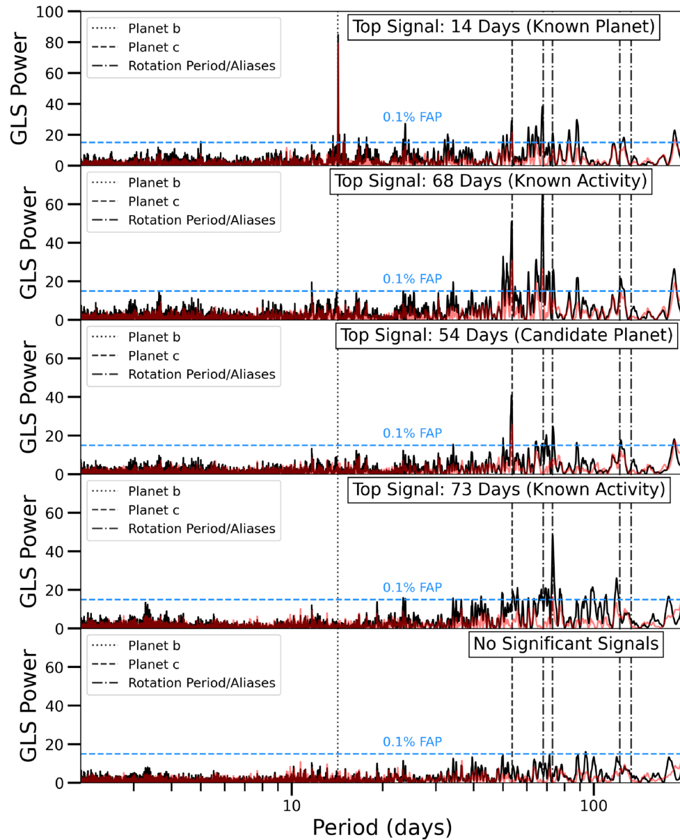
Figure 3. from Corey Beard et al 2025 Astron. J. 170 doi:10.3847/1538-3881/ae0e20 https://dx.doi.org/10.3847/1538-3881/ae0e20 © 2025. The Author(s). Published by the American Astronomical Society.
