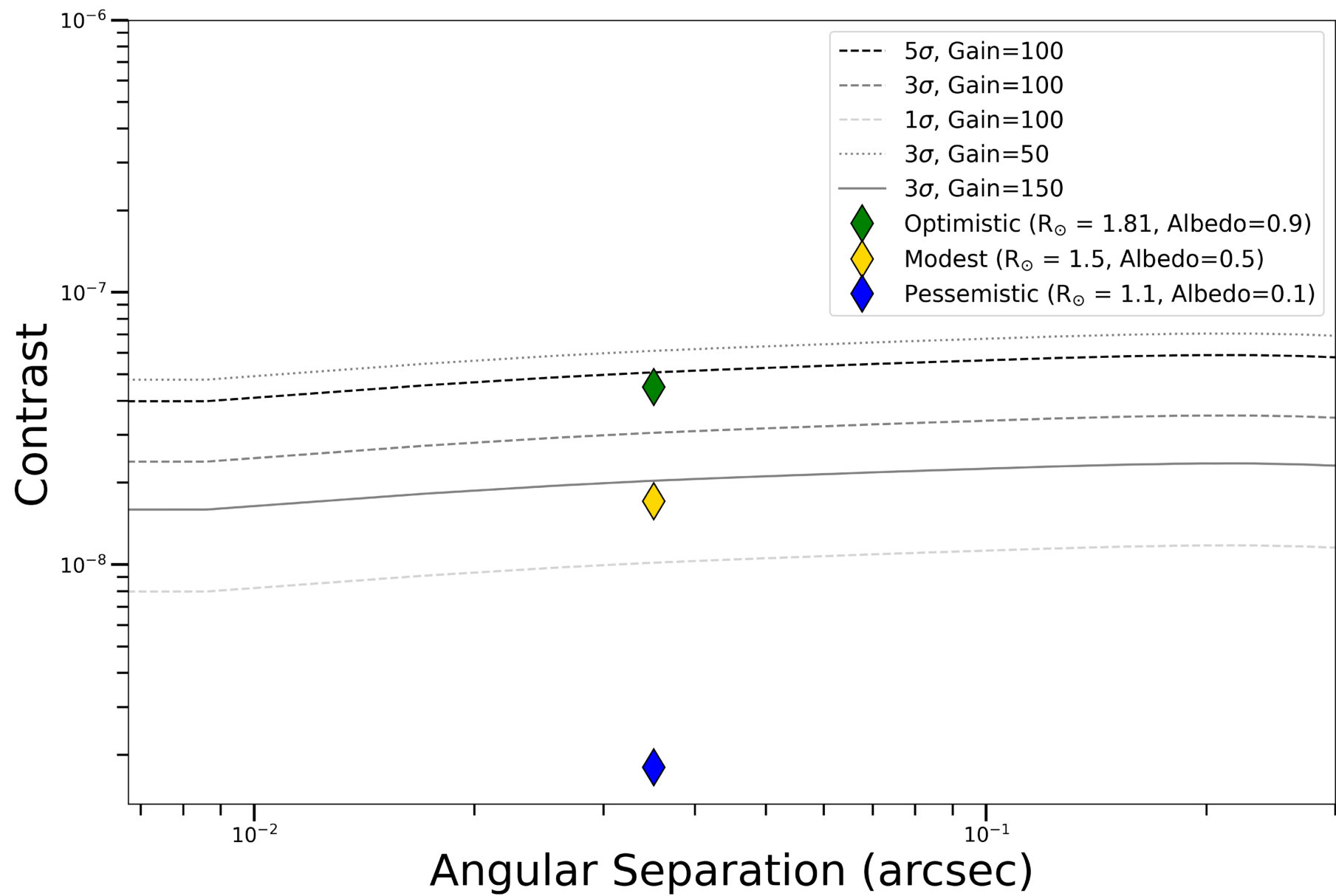
Figure B1. from Corey Beard et al 2025 Astron. J. 170 doi:10.3847/1538-3881/ae0e20 https://dx.doi.org/10.3847/1538-3881/ae0e20 © 2025. The Author(s). Published by the American Astronomical Society.
