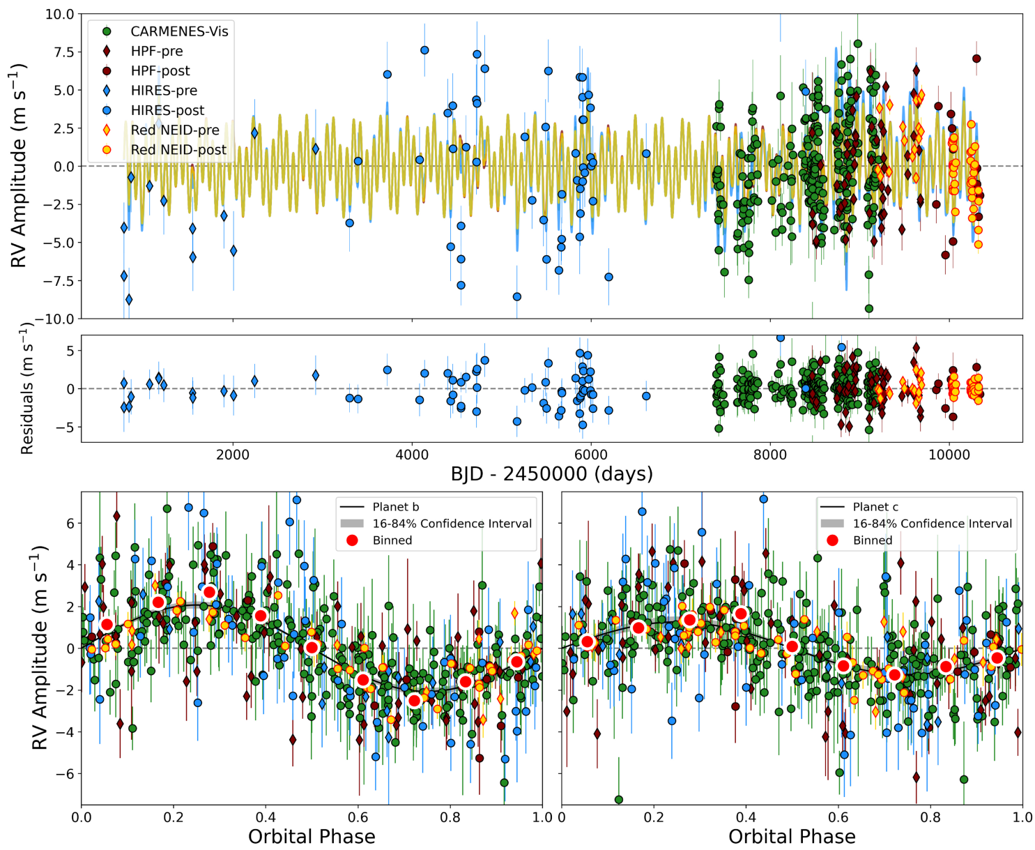
Figure A3. from Corey Beard et al 2025 Astron. J. 170 doi:10.3847/1538-3881/ae0e20 https://dx.doi.org/10.3847/1538-3881/ae0e20 © 2025. The Author(s). Published by the American Astronomical Society.
