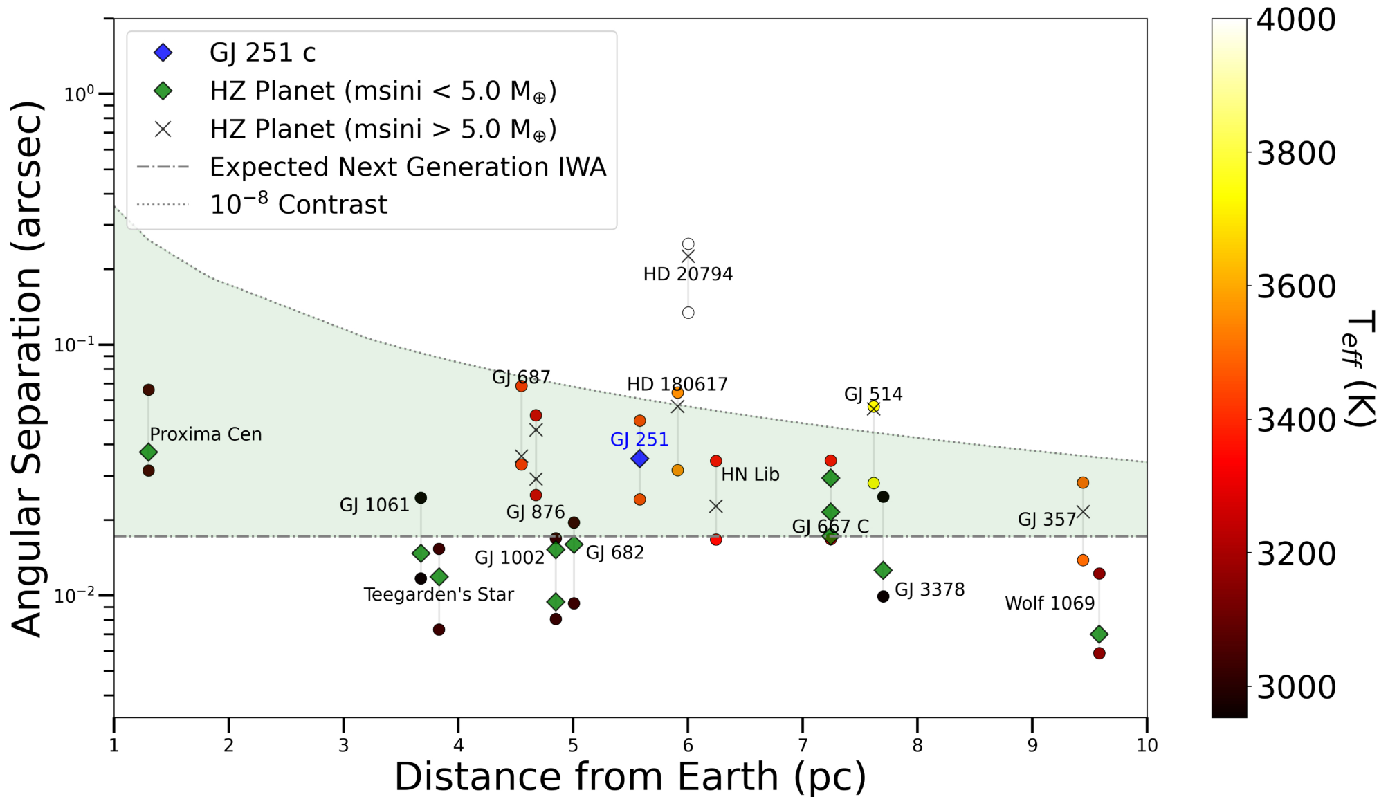
Figure 14. from Corey Beard et al 2025 Astron. J. 170 doi:10.3847/1538-3881/ae0e20 https://dx.doi.org/10.3847/1538-3881/ae0e20 © 2025. The Author(s). Published by the American Astronomical Society.
