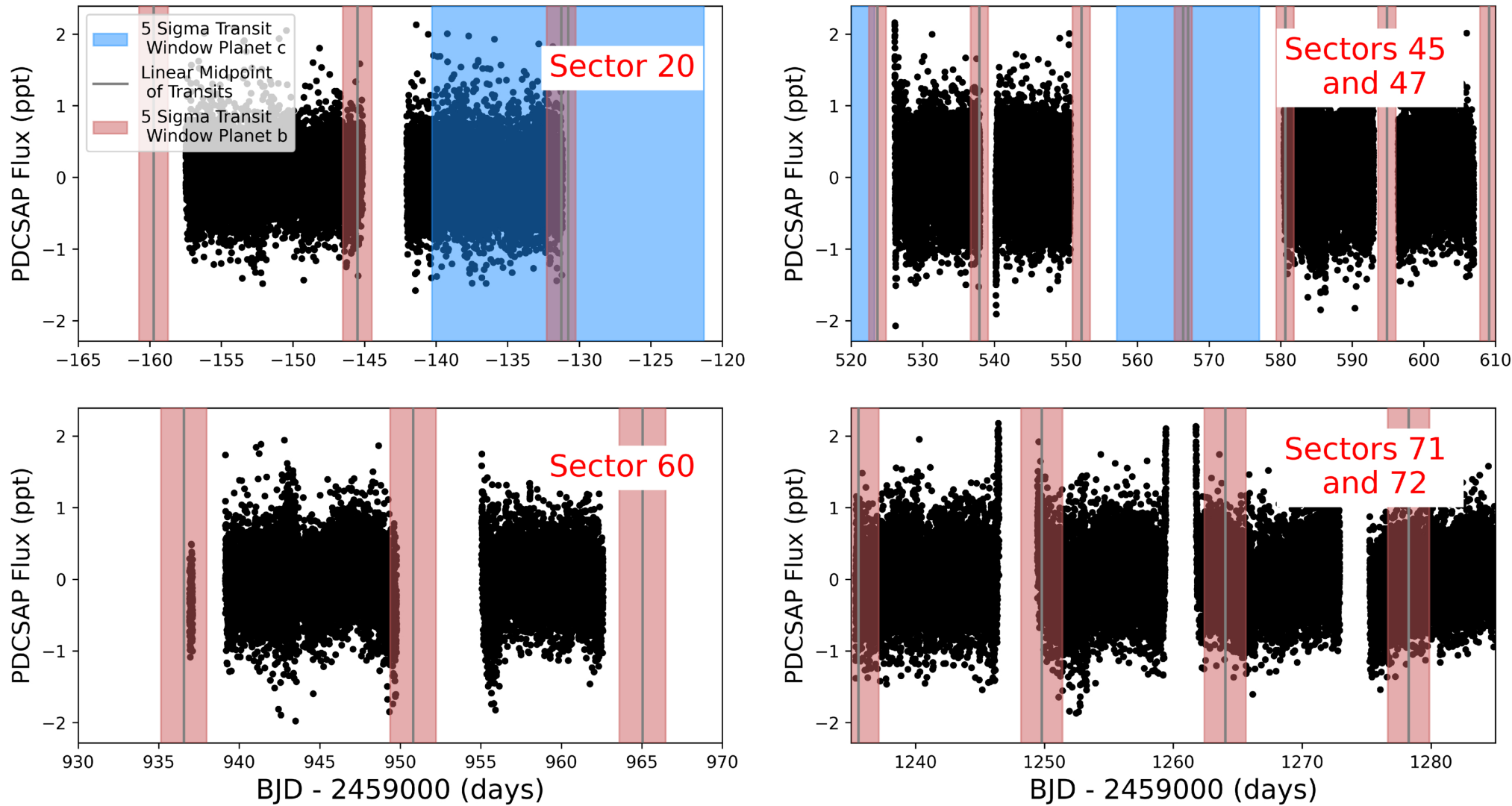
Figure 12. from Corey Beard et al 2025 Astron. J. 170 doi:10.3847/1538-3881/ae0e20 https://dx.doi.org/10.3847/1538-3881/ae0e20 © 2025. The Author(s). Published by the American Astronomical Society.
