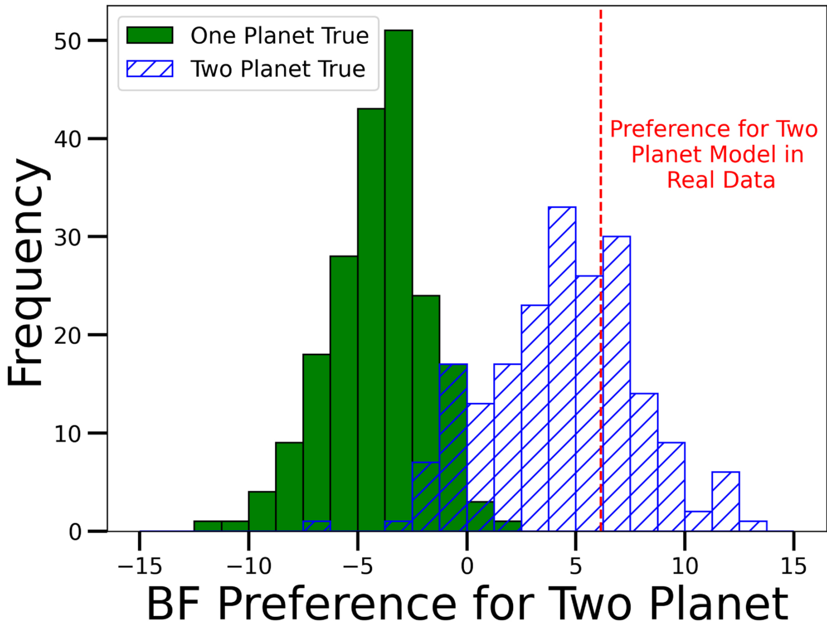
Figure 10. from Corey Beard et al 2025 Astron. J. 170 doi:10.3847/1538-3881/ae0e20 https://dx.doi.org/10.3847/1538-3881/ae0e20 © 2025. The Author(s). Published by the American Astronomical Society.
