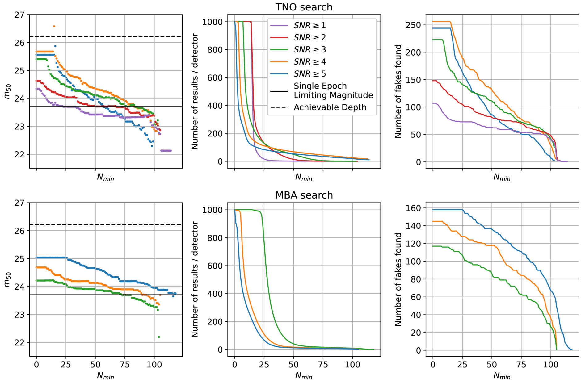
Figure 7. from Steven Stetzler et al 2025 Astron. J. 170 doi:10.3847/1538-3881/ae0e1a https://dx.doi.org/10.3847/1538-3881/ae0e1a © 2025. The Author(s). Published by the American Astronomical Society.
