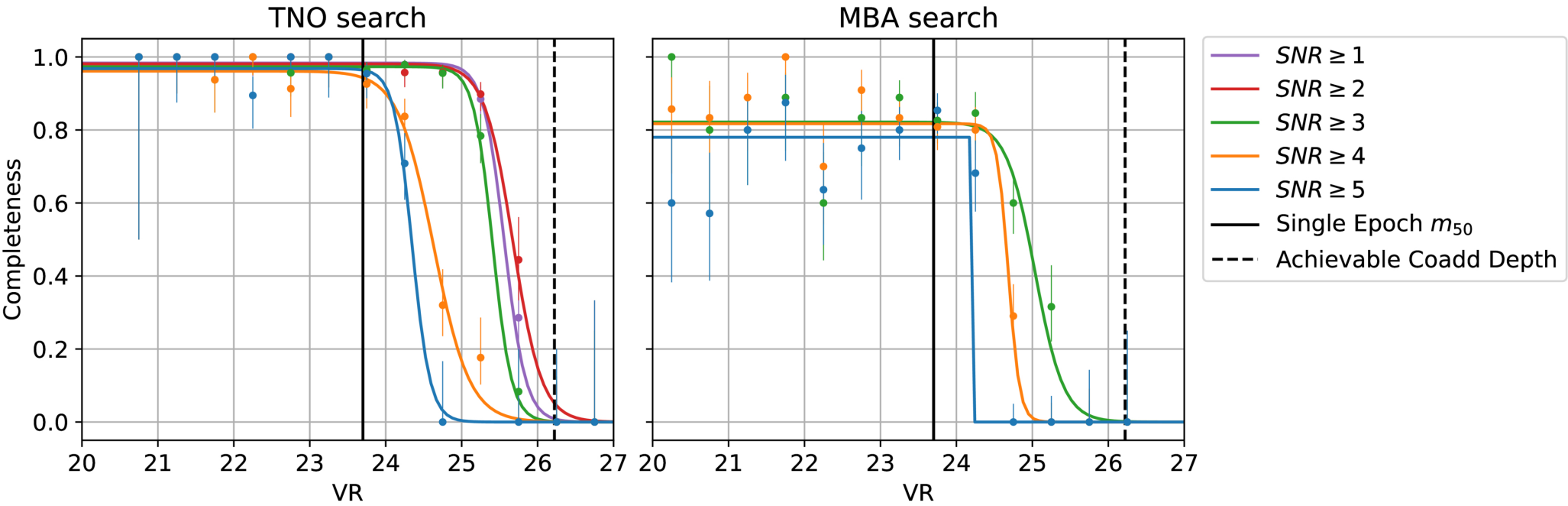
Figure 6. from Steven Stetzler et al 2025 Astron. J. 170 doi:10.3847/1538-3881/ae0e1a https://dx.doi.org/10.3847/1538-3881/ae0e1a © 2025. The Author(s). Published by the American Astronomical Society.
