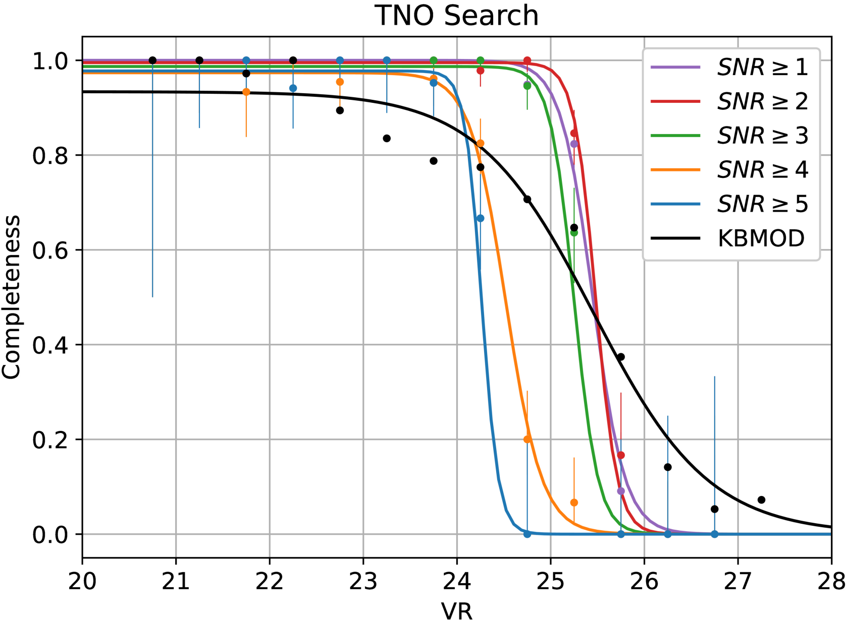
Figure 12. from Steven Stetzler et al 2025 Astron. J. 170 doi:10.3847/1538-3881/ae0e1a https://dx.doi.org/10.3847/1538-3881/ae0e1a © 2025. The Author(s). Published by the American Astronomical Society.
