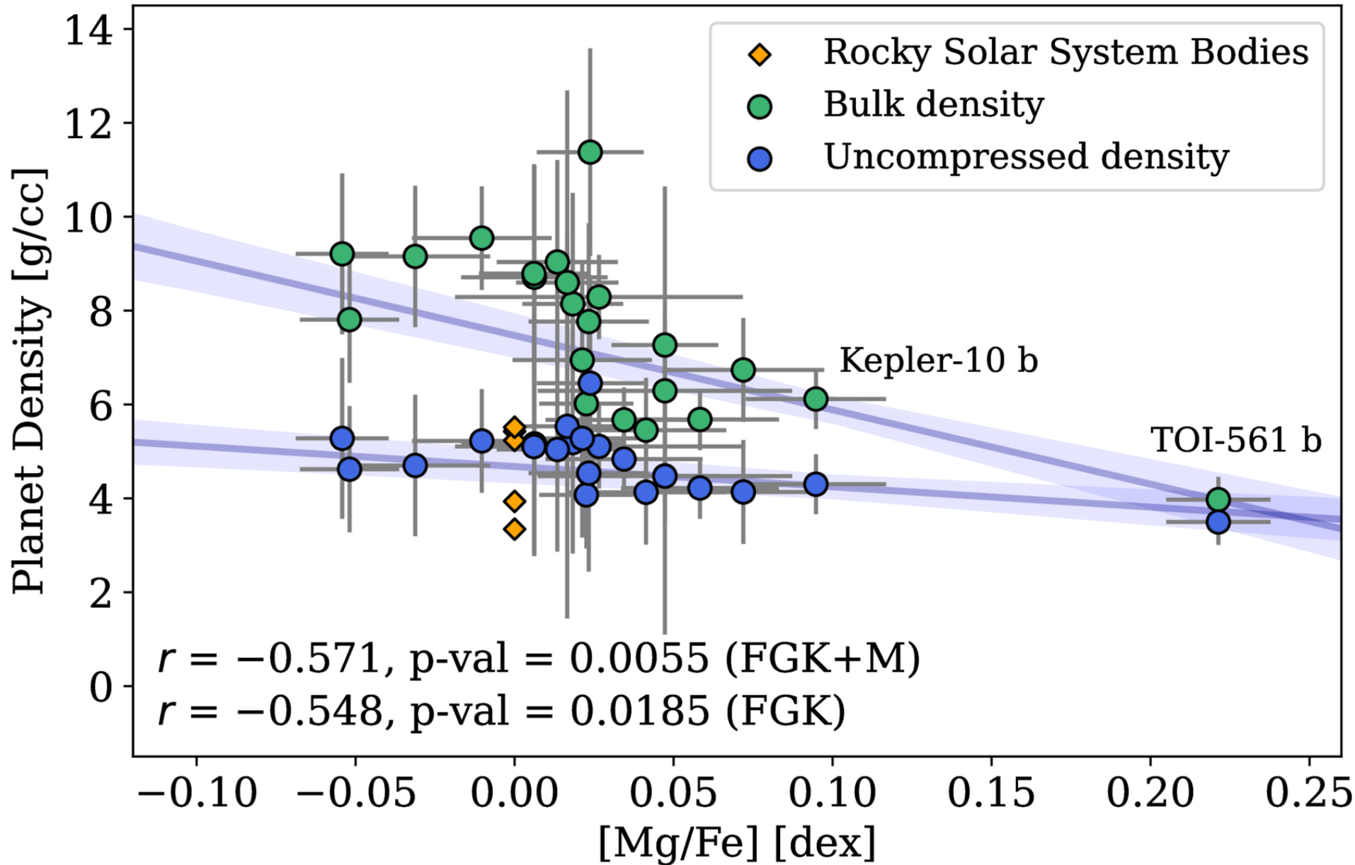
Figure 6. from Aida Behmard et al 2025 Astron. J. 170 doi:10.3847/1538-3881/ae0e17 https://dx.doi.org/10.3847/1538-3881/ae0e17 © 2025. The Author(s). Published by the American Astronomical Society.
