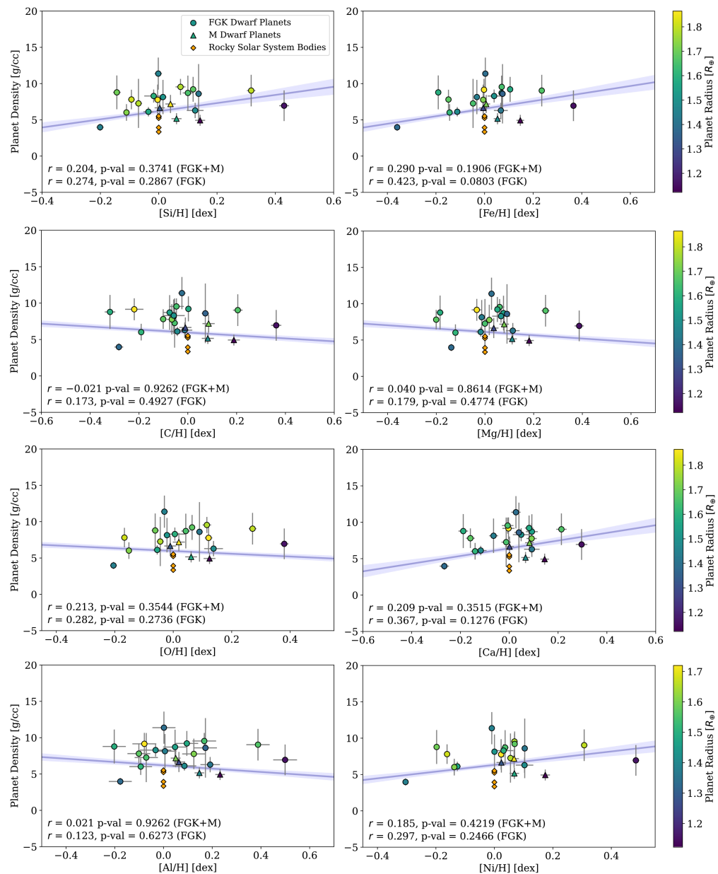
Figure 3. from Aida Behmard et al 2025 Astron. J. 170 doi:10.3847/1538-3881/ae0e17 https://dx.doi.org/10.3847/1538-3881/ae0e17 © 2025. The Author(s). Published by the American Astronomical Society.
