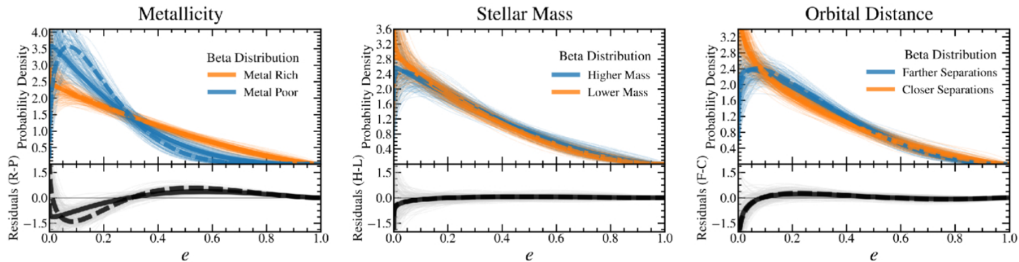
Figure 7. from Marvin Morgan et al 2026 Astron. J. 171 doi:10.3847/1538-3881/ae0e16 https://dx.doi.org/10.3847/1538-3881/ae0e16 © 2025. The Author(s). Published by the American Astronomical Society.
