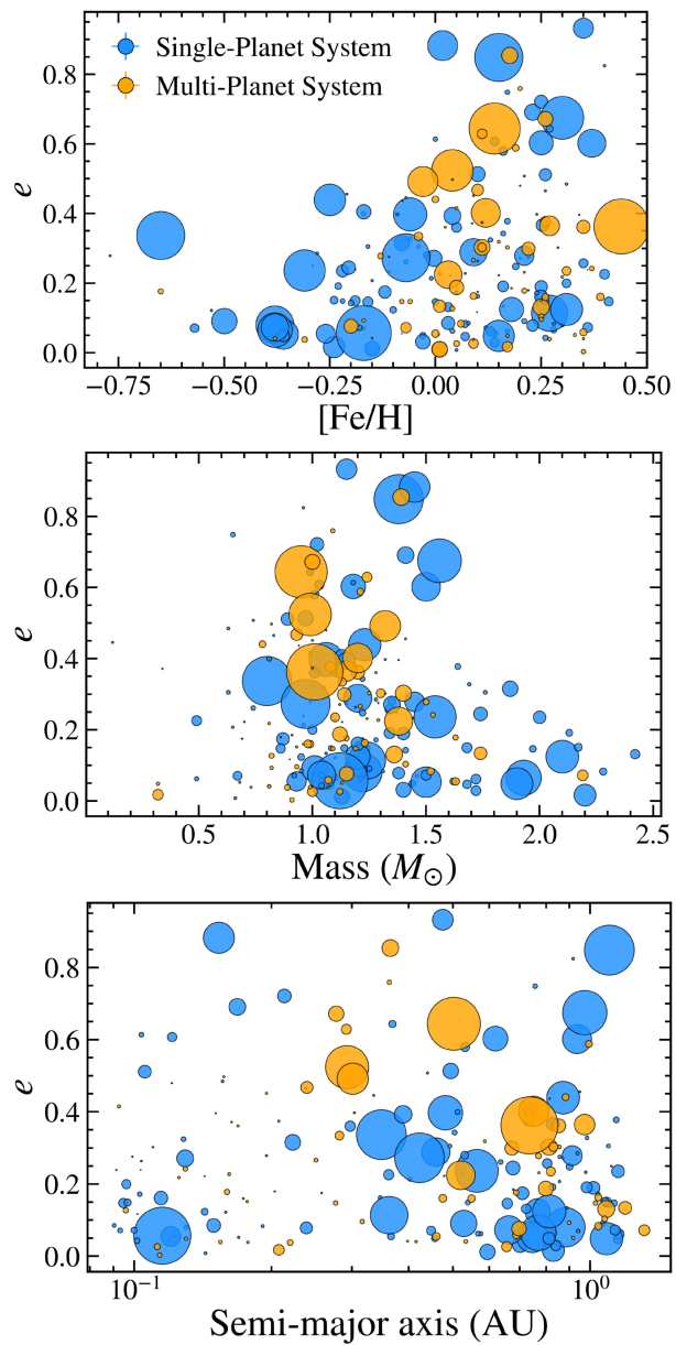
Figure 6. from Marvin Morgan et al 2026 Astron. J. 171 doi:10.3847/1538-3881/ae0e16 https://dx.doi.org/10.3847/1538-3881/ae0e16 © 2025. The Author(s). Published by the American Astronomical Society.
