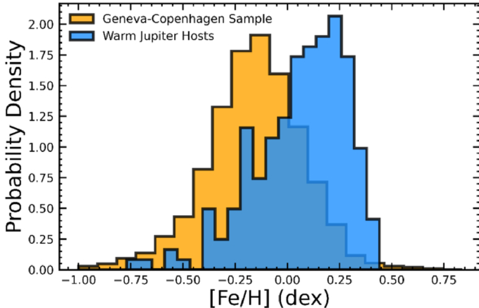
Figure 3. from Marvin Morgan et al 2026 Astron. J. 171 doi:10.3847/1538-3881/ae0e16 https://dx.doi.org/10.3847/1538-3881/ae0e16 © 2025. The Author(s). Published by the American Astronomical Society.
