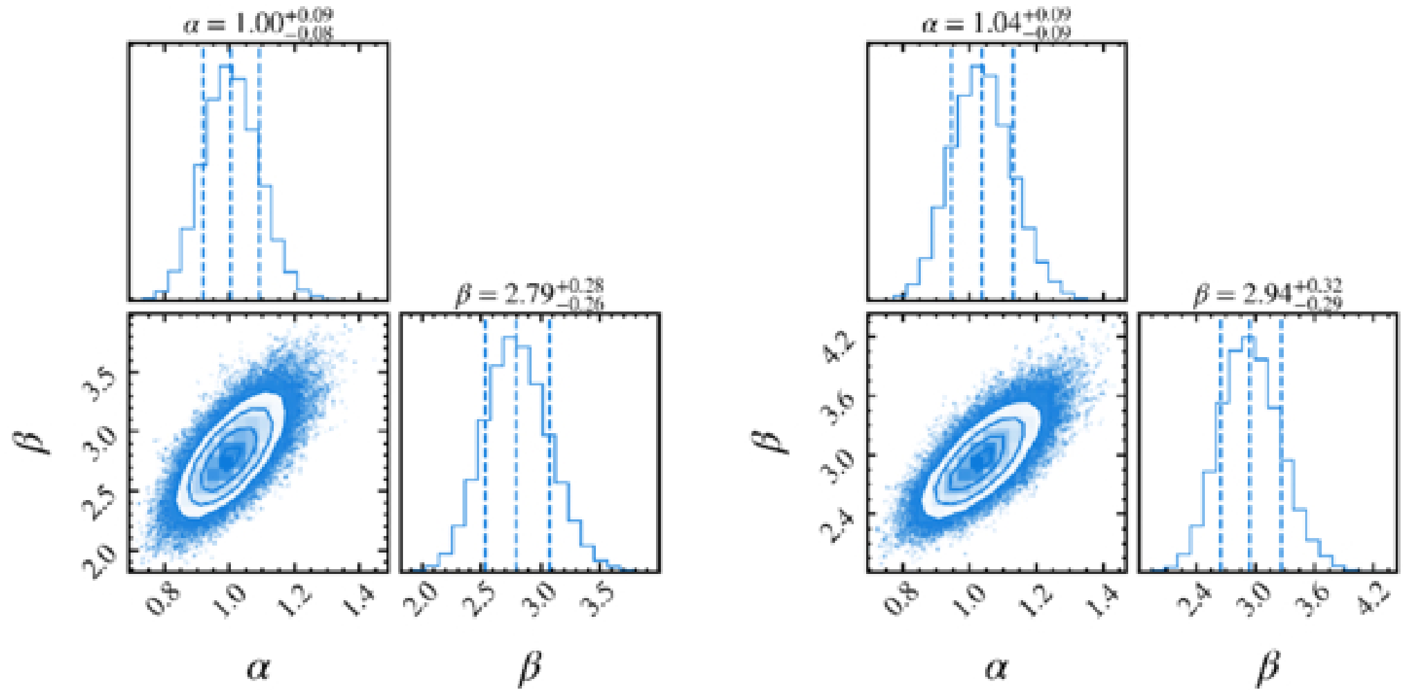
Figure 11. from Marvin Morgan et al 2026 Astron. J. 171 doi:10.3847/1538-3881/ae0e16 https://dx.doi.org/10.3847/1538-3881/ae0e16 © 2025. The Author(s). Published by the American Astronomical Society.
