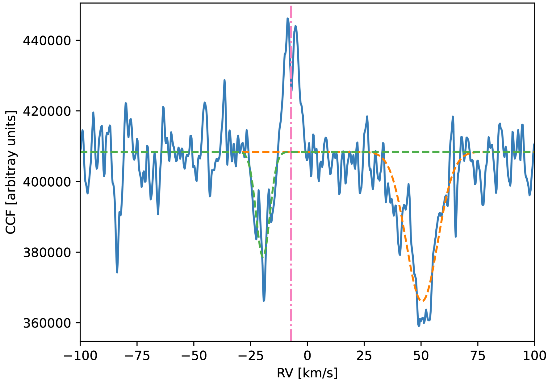
Figure 3. from Sean M. O'Brien et al 2025 Astron. J. 170 doi:10.3847/1538-3881/ae0e0d https://dx.doi.org/10.3847/1538-3881/ae0e0d © 2025. The Author(s). Published by the American Astronomical Society.
