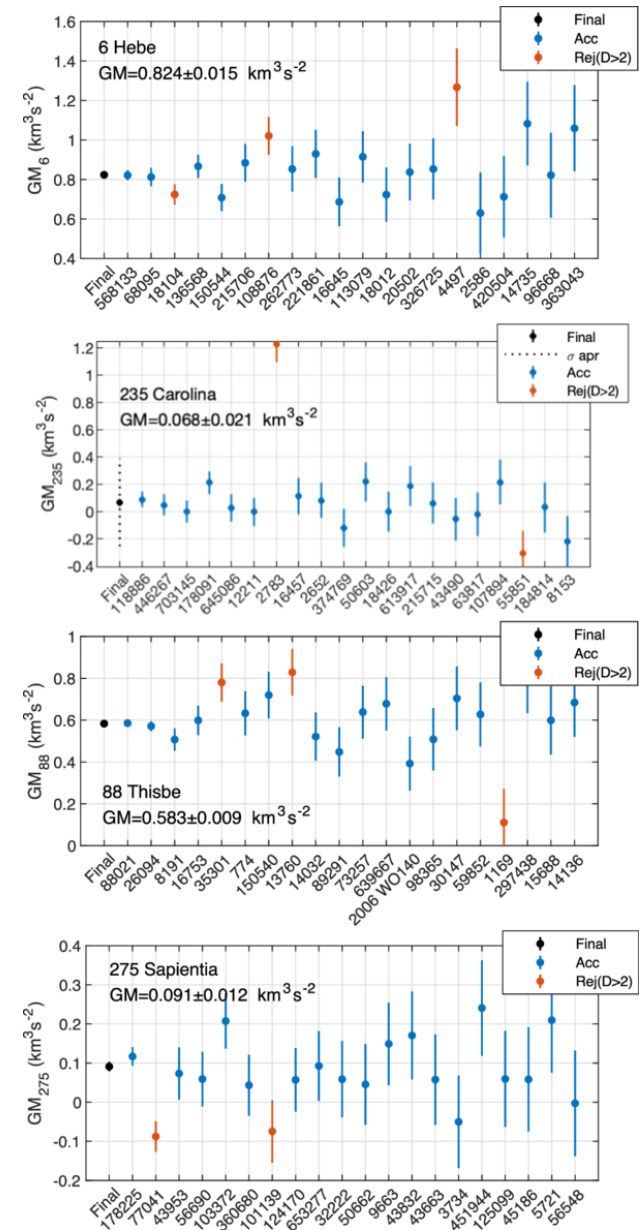
Figure 5. from Oscar Fuentes-Muñoz et al 2025 Astron. J. 170 doi:10.3847/1538-3881/ae0cc9 https://dx.doi.org/10.3847/1538-3881/ae0cc9 © 2025. The Author(s). Published by the American Astronomical Society.
