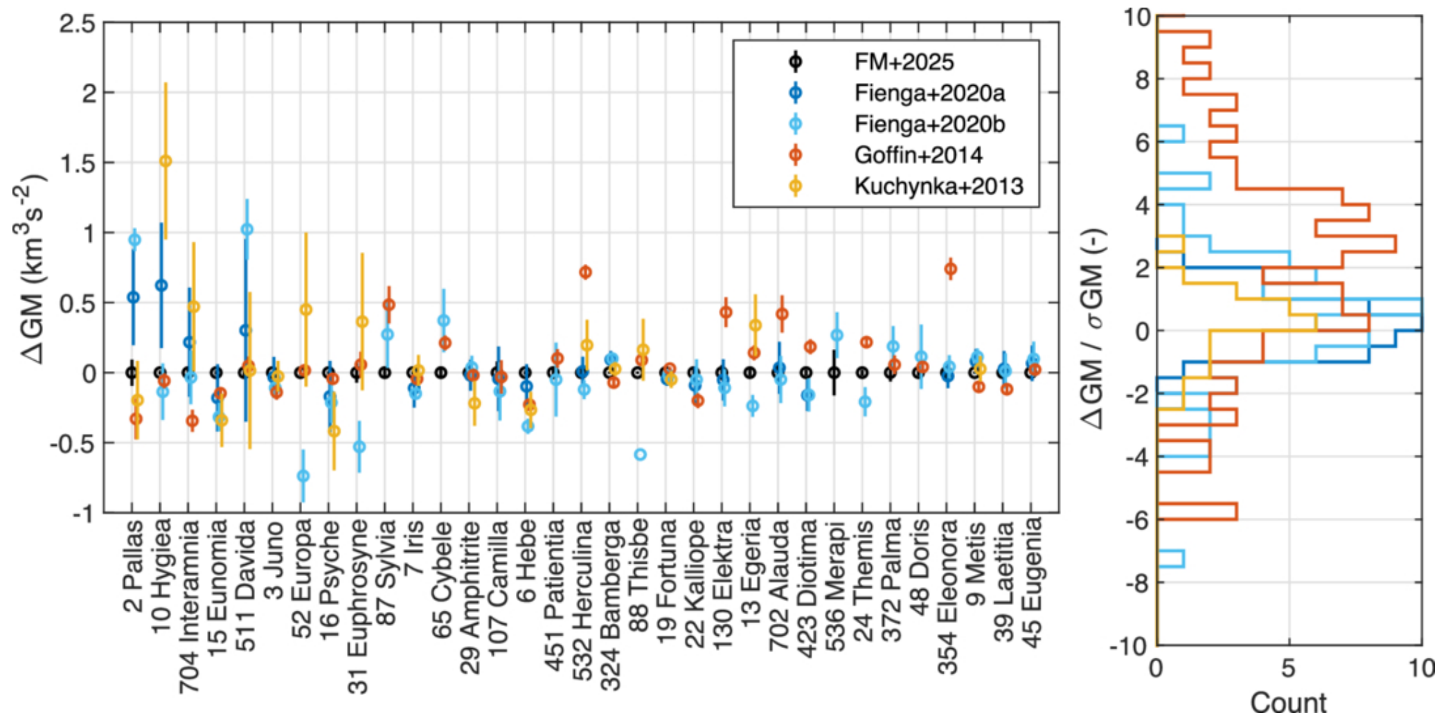
Figure 15. from Oscar Fuentes-Muñoz et al 2025 Astron. J. 170 doi:10.3847/1538-3881/ae0cc9 https://dx.doi.org/10.3847/1538-3881/ae0cc9 © 2025. The Author(s). Published by the American Astronomical Society.
