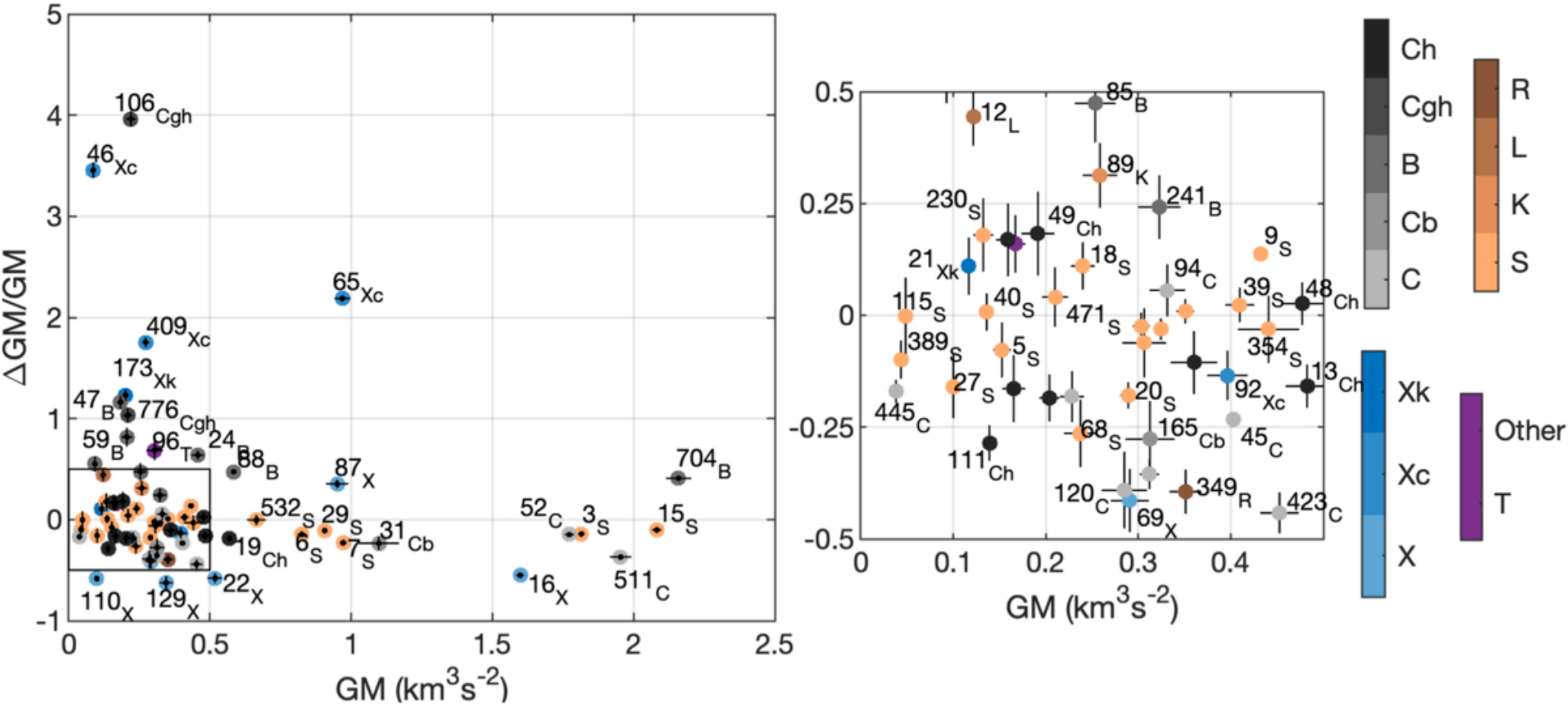
Figure 11. from Oscar Fuentes-Muñoz et al 2025 Astron. J. 170 doi:10.3847/1538-3881/ae0cc9 https://dx.doi.org/10.3847/1538-3881/ae0cc9 © 2025. The Author(s). Published by the American Astronomical Society.
