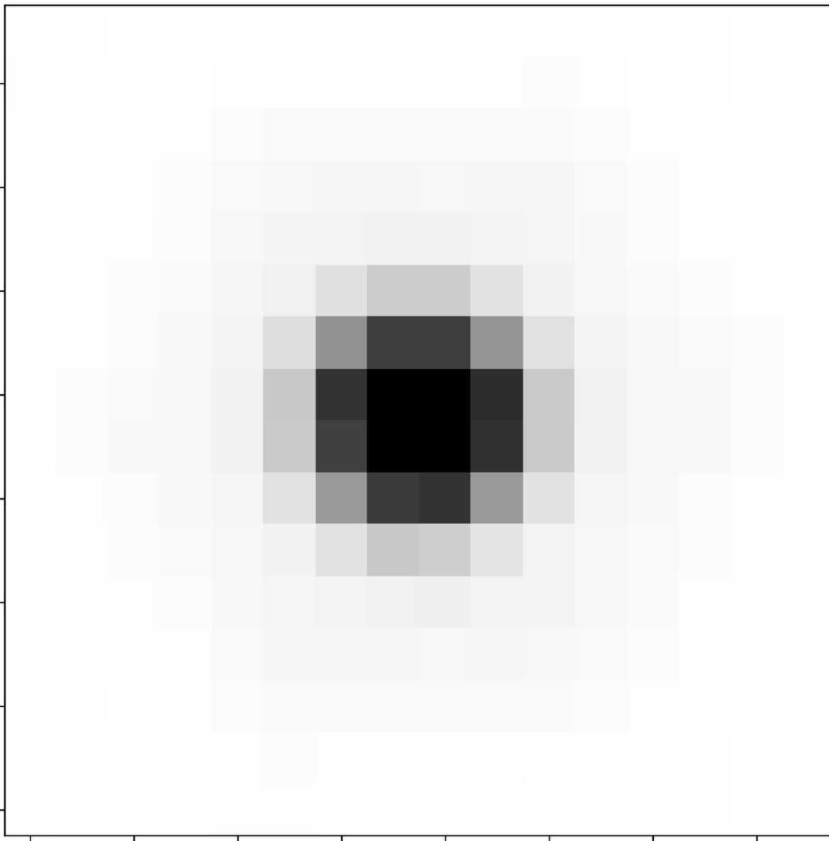
Figure 5. from Bren E. Backhaus et al 2025 Astron. J. 170 doi:10.3847/1538-3881/ae0cc4 https://dx.doi.org/10.3847/1538-3881/ae0cc4 © 2025. The Author(s). Published by the American Astronomical Society.
