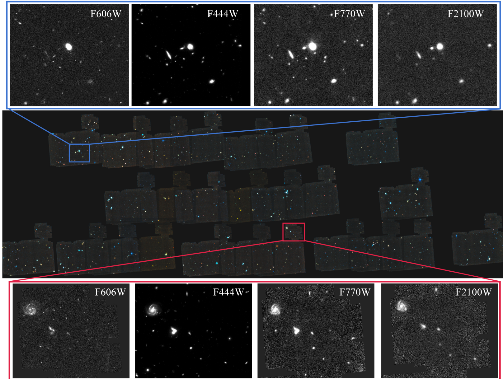
Figure 3. from Bren E. Backhaus et al 2025 Astron. J. 170 doi:10.3847/1538-3881/ae0cc4 https://dx.doi.org/10.3847/1538-3881/ae0cc4 © 2025. The Author(s). Published by the American Astronomical Society.
