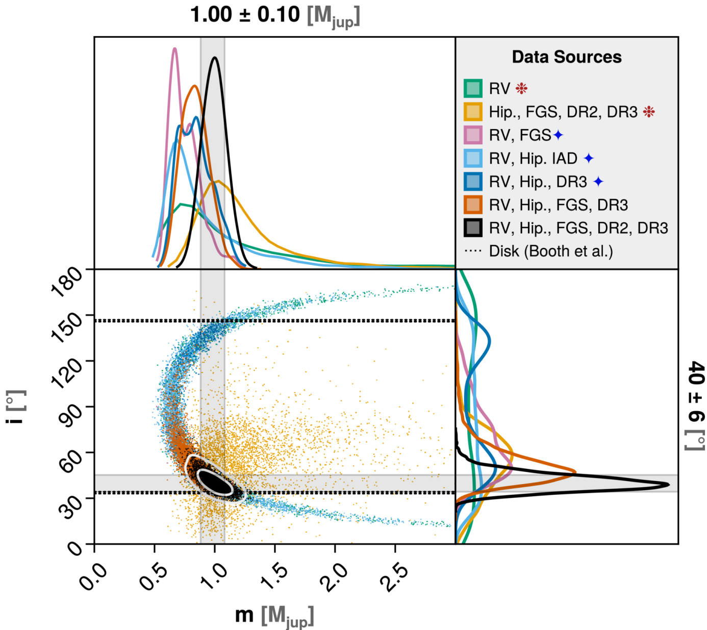
Figure 9. from William Thompson et al 2025 Astron. J. 170 doi:10.3847/1538-3881/ae0cbd https://dx.doi.org/10.3847/1538-3881/ae0cbd © 2025. The Author(s). Published by the American Astronomical Society.
