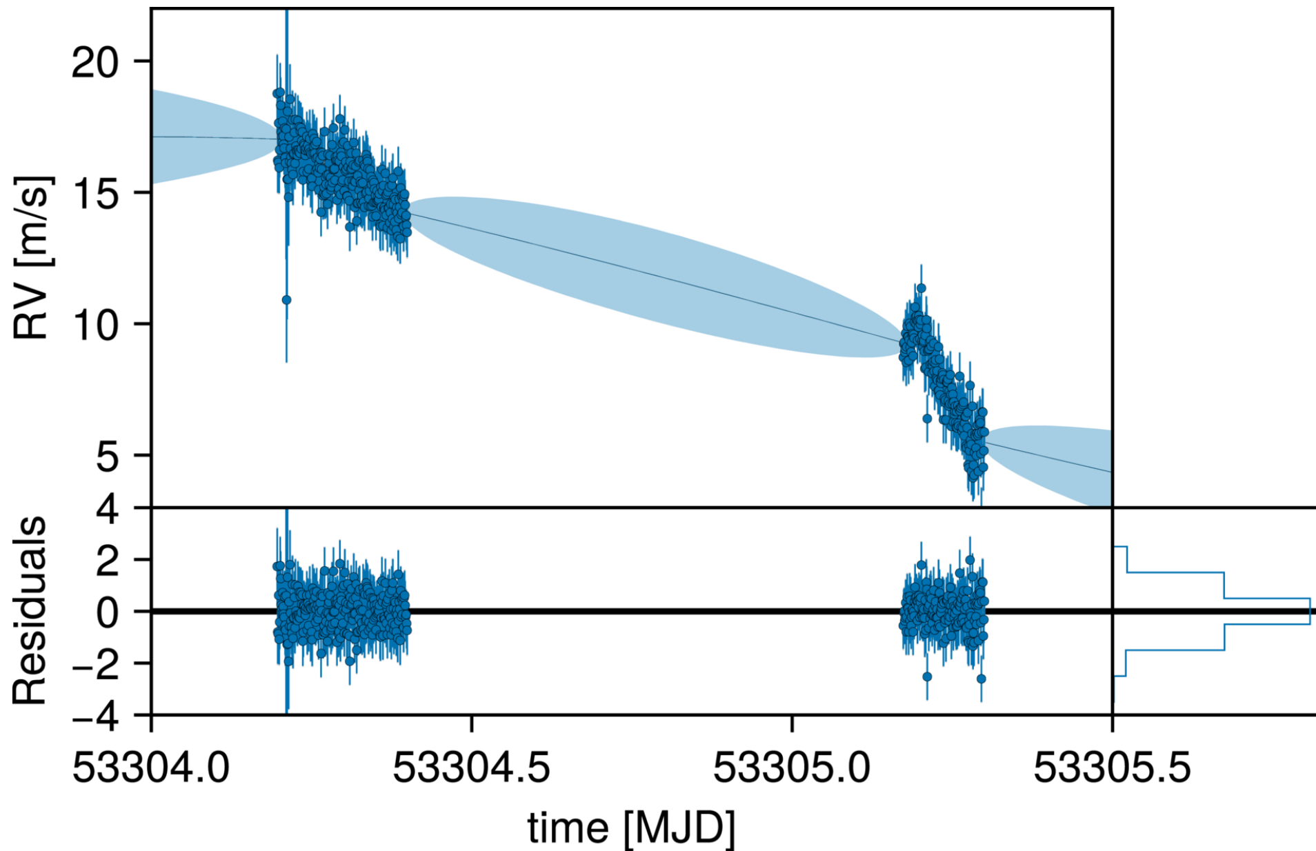
Figure 8. from William Thompson et al 2025 Astron. J. 170 doi:10.3847/1538-3881/ae0cbd https://dx.doi.org/10.3847/1538-3881/ae0cbd © 2025. The Author(s). Published by the American Astronomical Society.
