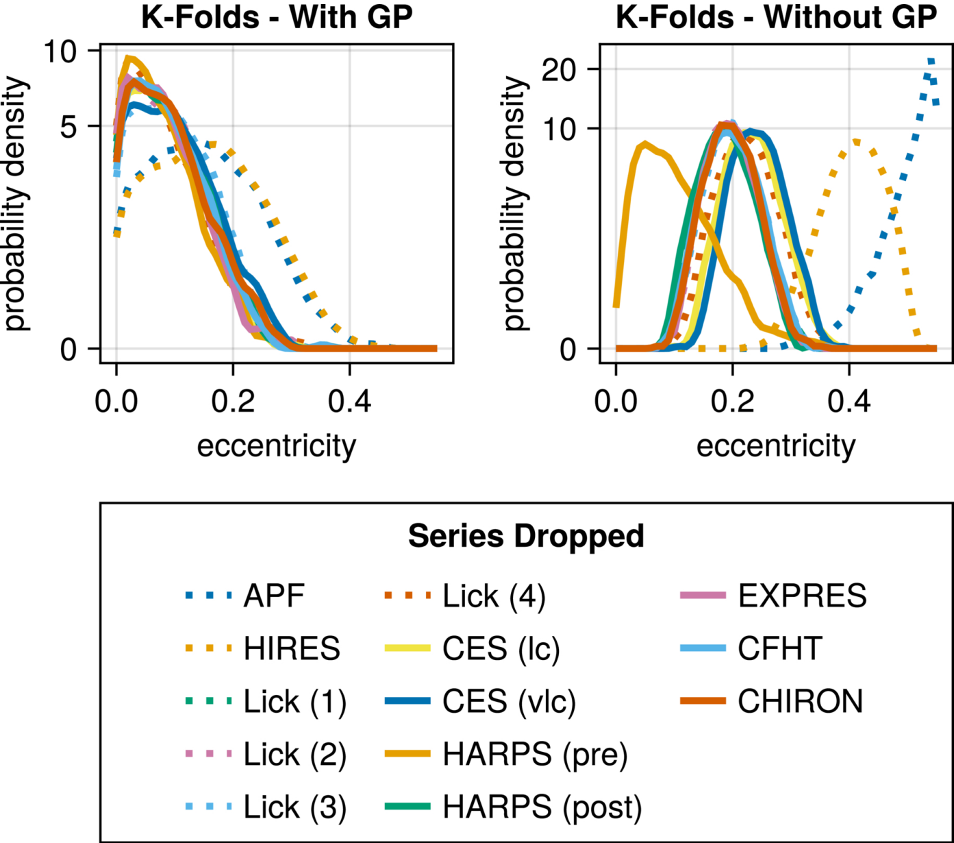
Figure 7. from William Thompson et al 2025 Astron. J. 170 doi:10.3847/1538-3881/ae0cbd https://dx.doi.org/10.3847/1538-3881/ae0cbd © 2025. The Author(s). Published by the American Astronomical Society.
